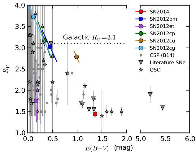
Figure 18. Fitted R_V and E(B - V) for the full phase range of -10 to +35 days, where SN2011by has been used as reference for SNe 2012bm, 2012cg, and 2012cp and SN2011fe was used for the remaining SNe. Also plotted are measurements from the literature, where 9 SNe Ia from Hernandez et al. (2000); Krisciunas et al. (2006, 2007); Benetti et al. (2004); Elias-Rosa et al. (2006, 2008); Hicken et al. (2009) and Folatelli et al. (2010) together with three Type II SNe from Pozzo et al. (2006) and Poznanski et al. (2009) are included. The parameters measured by studying reddening of QSO by foreground galaxies are from Elíasdóttir et al. (2006) and Östman, Goobar & Mörtzell (2006).
