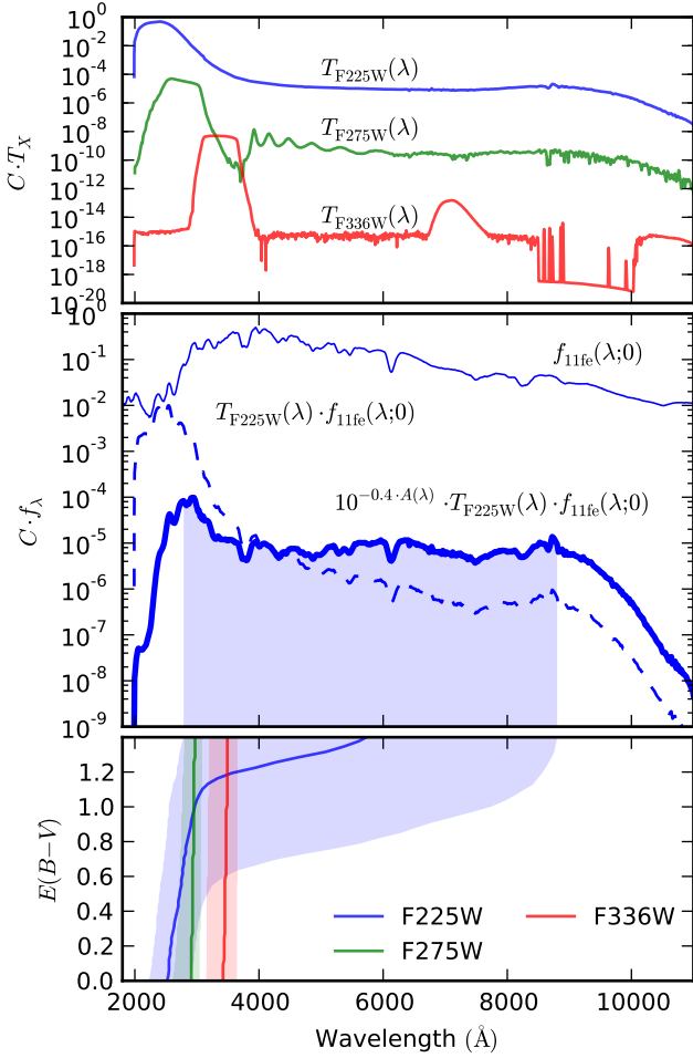
Figure D1. The upper panel shows the filter transmissions, T_X(\lambda) , of the WFC3/UVIS passbands, multiplied by an arbitrary normalisation, C . The thin, blue, line in the middle panel shows the spectrum of SN 2011fe at B band maximum, while the dashed, blue, line shows the same spectrum after it has been multiplied by the F225W throughput. The thick, blue, line shows the same spectrum after it has been reddened with a F99 extinction law with E(B - V) = 1.4 mag and R_V = 1.4 , similar to what we observe for SN 2014J. All three spectra have arbitrary normalisation, C . In the plot we have also marked the wavelength region from which 80 % of the light originates from, defined such that 10 % of light comes from bluer wavelengths, and 10 % comes from redder wavelengths. The lower panel shows the median wavelength, i.e. where 50 % of the light originates from redder and bluer wavelengths, for three passbands for SN 2011fe at B maximum, reddened with a F99 extinction law ( R_V = 1.4 ) with increasing extinction. The 80 % region is shown in the same manner as for the middle panel.
