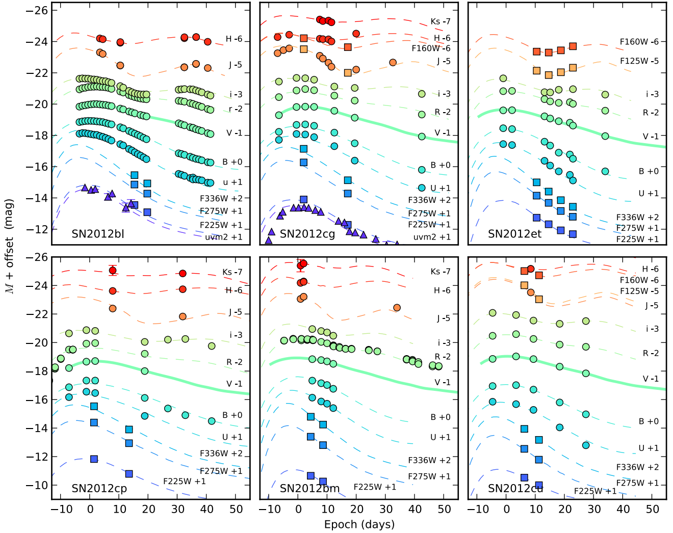
Figure 3. Observed light curves for the SN sample. Our analysis is based on optical UBVRI and NIR JHK photometry from ground based observatories (circles), UV (F225W, F275W, F336W) and NIR (F125W, F160W) photometry from the HST (squares). For the SNe 2012bl and 2012cg we also use Swift / UVOT photometry (triangles). The data are shown in their instrumental system but have been shifted using the distance moduli based on the distances in Table 1 and offset for clarity. The thick, solid, lines show the SNooPy V-models used to calculate colours as described in the text, while the dashed lines show synthesised light curves of SN2011fe to guide the eye. When a SN has observations in a similar filter from multiple instruments only one of the light curves is shown. The epoch is the observed date with respect to the fitted day of maximum in the B -band from Table 5.
