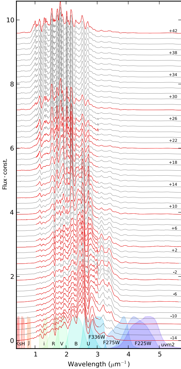
Figure B1. The spectral template constructed from measured spectra of SN 2011fe. Sections based on measured data are shown in red, while the interpolated sections, warped to the light curve are shown in grey. The filters used for the warping are shown at the bottom of the figure.
