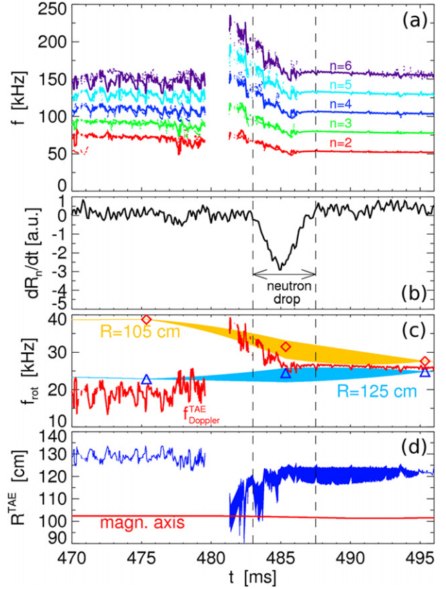
Figure 19. (a) Measured (dots) and reconstructed (solid line) frequencies for n = 2, \dots, 6 TAEs. Reconstruction is obtained from f_0^{TAE} and f_{Doppler}^{TAE} resulting from a linear fit of the measured f_{lab,n}^{TAE} = f_{lab,n}^{TAE}(n) . (b) Time derivative of the neutron rate. The negative dip, delimited by vertical dashed lines, indicates when fast ions are expelled from the plasma, possibly causing a transient drop in the toroidal rotation. (c) Measured rotation, with integration time of \sim 10 ms, at the plasma centre (diamonds) and at mid-radius (triangles). Shaded regions indicate different interpolations of the rotation evolution during the avalanche over short time scales. The maximum deviation around the measured values is \pm 10\% . f_{Doppler}^{TAE} is also shown for reference. (d) Sensitivity of the inferred R^{TAE} upon toroidal velocity evolution within the values in panel (c).
