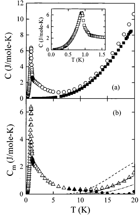
FIG. 6. (a) Heat capacity C(T) of CePtPb and LaPtPb for 0.2 < T < 20 K. Inset: C(T) for CePtPb in the region of the antiferromagnetic transition, showing a peak at T_N = 0.9 K. (b) The magnetic specific heat C_m = C(\text{CePtPb}) - C(\text{LaPtPb}) . The lines show the expected contribution from a crystal-field doublet located at an energy k_B\delta above the ground doublet. The value \delta = 100 K gives the best representation of the data. The solid circles represent the magnetic specific heat after subtraction of the contribution of the higher doublet, with \delta = 100 K. The contribution of the ground-state doublet is seen to be highly asymmetric above and below T_N , and to extend to very high temperatures ( 15 K) relative to T_N .
