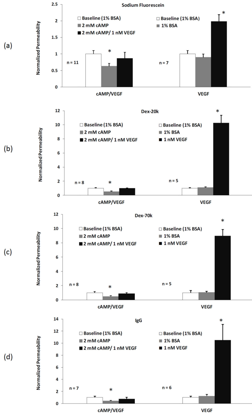
Figure 6. Comparison of apparent P (mean \pm SE) in the test group (20 min pretreatment with cAMP and then VEGF/cAMP), left panel, and that in the control group (no cAMP), right panel, for (a) sodium fluorescein, (b) Dex-20k, (c) Dex-70k, and (d) IgG. The first bar in each group is the baseline with 1% BSA Ringer perfusion, the second bar in the test group is P after 20 min cAMP treatment and the third bar is P after ~30 sec VEGF/cAMP treatment. For comparison, the second bar in the control group is P after 20 min 1% BSA Ringer and the
