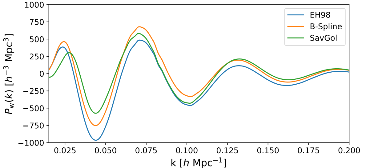
Figure 11. The linear wiggly power spectrum for three choices of P_{\text{nw}} . The conventional choice (EH98 [60]) does not accurately capture the large scale power, and we have investigated two possible methods to mitigate this discrepancy: one based on B-splines, described in ref. [61] and another based on a Savitsky-Golay filter in \ln(k) . The wiggly power spectra isolated using these three methods exhibit visibly different oscillatory behavior.
