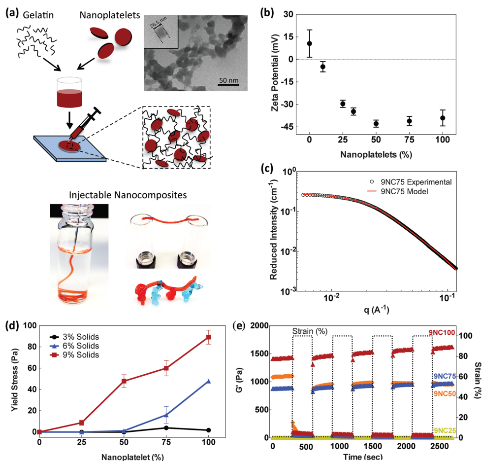
Figure 1. Structure, injectability, and self-healing characteristics of nanocomposite hydrogels. (a) Schematic showing the preparation of the nanocomposite gels. The TEM image shows the size of the silicate nanoparticle (scale bar 50 nm). Images showing injection of nanocomposite hydrogel through a surgical needle (22 gauge) and recovery to form freestanding structures. (b) Zeta potential measurements demonstrate electrostatic interactions between negatively charged silicate and positively charged gelatin; 95% CI are shown for each point. (c) Small-angle X-ray scattering (SAXS) indicates that nanoplatelets are well dispersed and follow the model curve for scattering from dispersed thin disks. (d) Yield stress of gels as a function of nanoplatelet loading and solids fraction. (e) Recovery of the nanocomposites was observed by subjecting the hydrogel to alternating high and low strain conditions (100% strain and 1% strain) while monitoring the moduli of the composite. For all the nanocomposite hydrogels, more than 95% recovery was observed.
