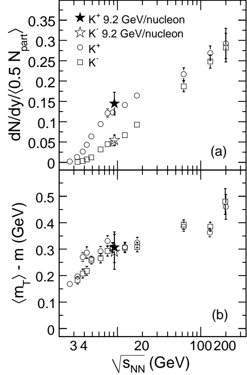
FIG. 18: (a) dN/dy normalized by \langle N_{\text{part}} \rangle / 2 and (b) \langle m_T \rangle - m of K^\pm , in 0-10% central Au+Au collisions for \sqrt{s_{NN}} = 9.2 GeV compared to previous results from AGS [38], SPS [39], and RHIC [23]. The errors shown are the quadrature sum of statistical and systematic uncertainties.
