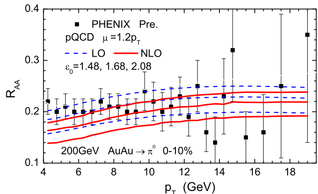
FIG. 1: Nuclear modification factors for \pi^0 spectra in LO (dashed) and NLO pQCD (solid) in Au + Au (0 – 10%) collisions at \sqrt{s} = 200 GeV with different values of energy loss parameter \epsilon_0 = 1.48, 1.68 and 2.08 GeV/fm (from top to bottom) compared with data [13].
