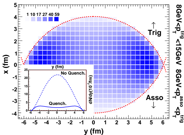
FIG. 5: The same as Fig. 2 except for dihadrons along the direction \phi = 0 and \pi .
