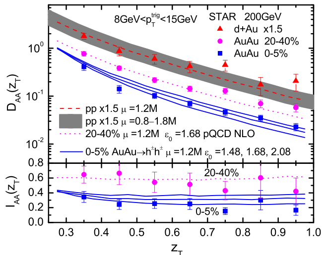
FIG. 4: Hadron-triggered fragmentation functions D_{AA}(z_T) and the medium modification factors I_{AA}(z_T) in NLO pQCD as compared to the data [15].
