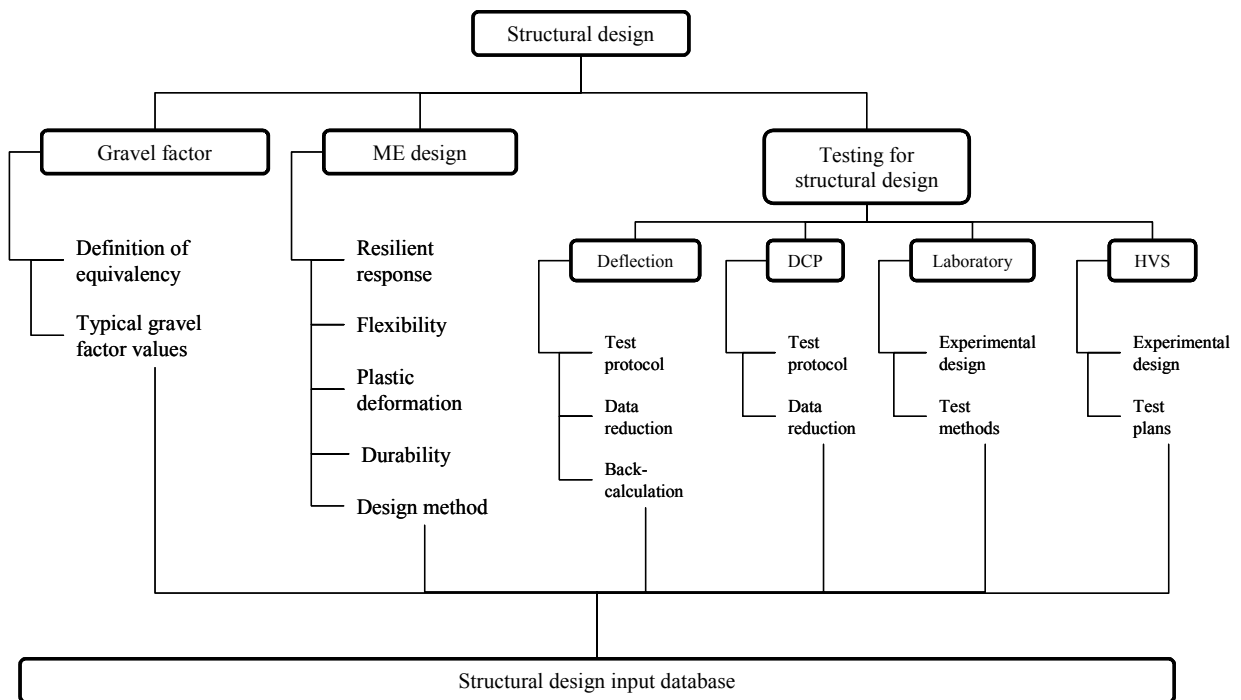
Figure 6. Structural design.
