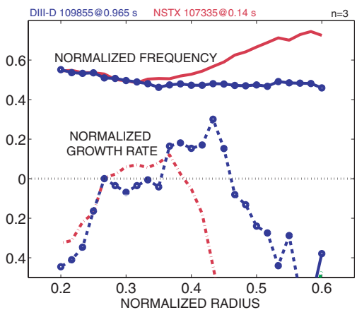
Figure 16. Frequency and growth rate (normalized to the central Alfvén frequency v_A/qR ) for the DIII-D ( \circ , \bullet ) and NSTX (no symbols) cases versus the normalized square root of the toroidal flux as calculated by HINST for n = 3 .
