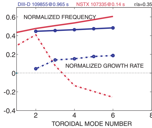
Figure 17. HINST calculation of frequency and growth rate for the DIII-D (○, ●) and NSTX (no symbols) cases versus toroidal mode number for a normalized radius of 0.35.
