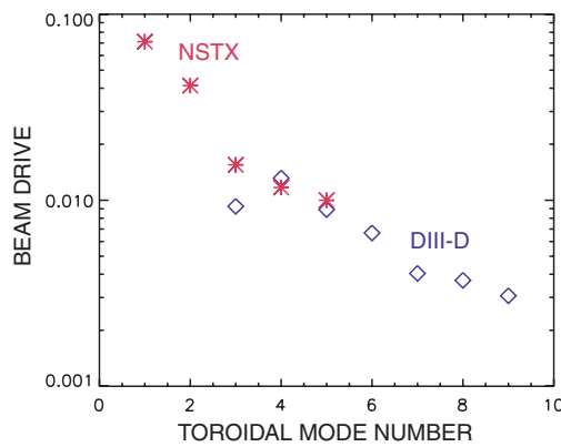
Figure 15. Beam ion drive for the most unstable TAE calculated by NOVA-K as a function of toroidal mode number for the NSTX ( \times ) and DIII-D ( \diamond ) cases shown in figure 13. The calculation includes finite drift orbit and finite gyroradius effects.
