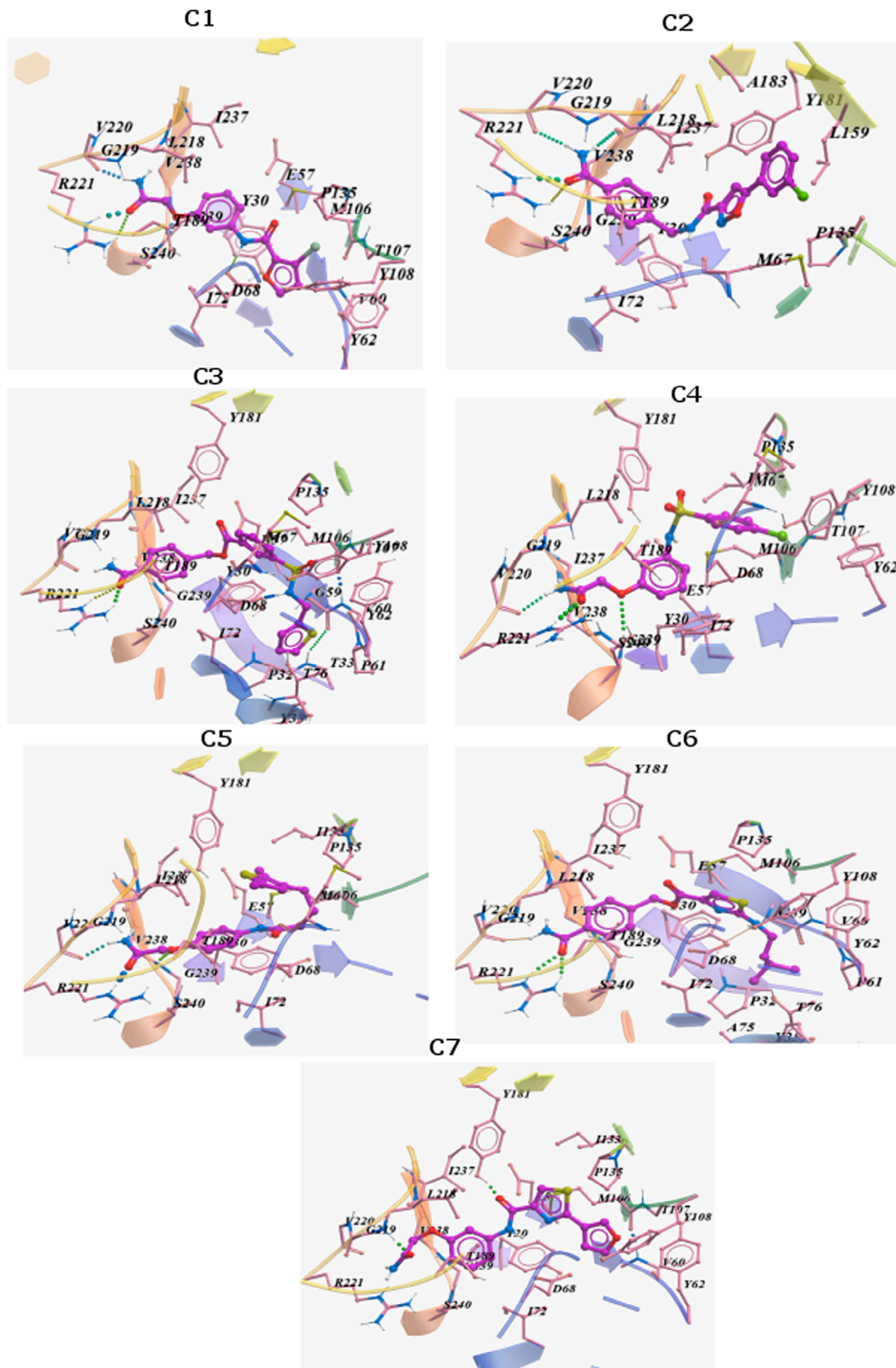
Figure 3. Binding interaction of candidate compounds (C1–C7) inside the binding pocket of homology model of \alpha -subunit of TRPS ( M. tuberculosis ).
