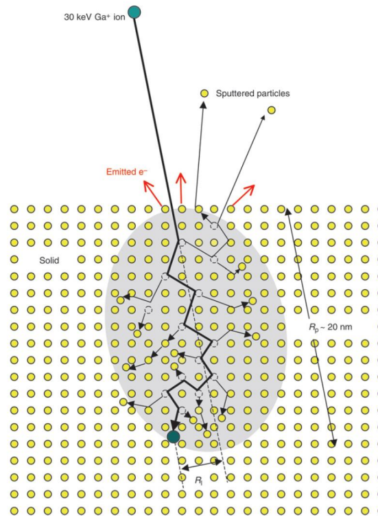
Figure 3.2 Schematic of a series of collisions generated by a 30 keV \text{Ga}^+ ion on a crystalline lattice. [21]
