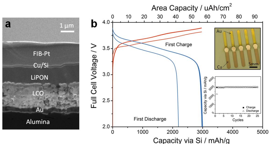
Figure 6.1 RF-magnetron sputtered all-solid-state batteries. a, Cross sectional ion-beam image of the solid-state battery shows all the solid-state components. b, The cycling profile of the solid-state batteries where the red lines denote charge profiles and the blue lines denote discharge profiles. The insets show the optical image of the solid-state batteries and the capacity vs. cycle over 25 cycles.
