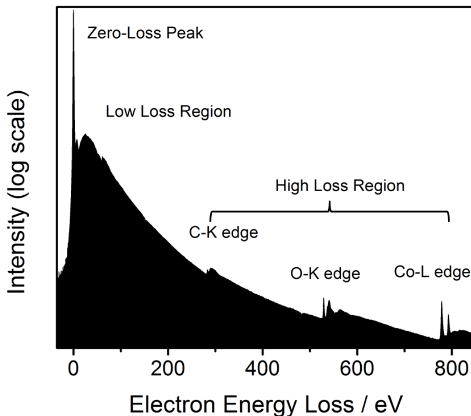
Figure 3.9 Electron energy loss spectrum of \text{LiCoO}_2 demonstrating typical features of a zero loss peak, low loss region and high loss region
