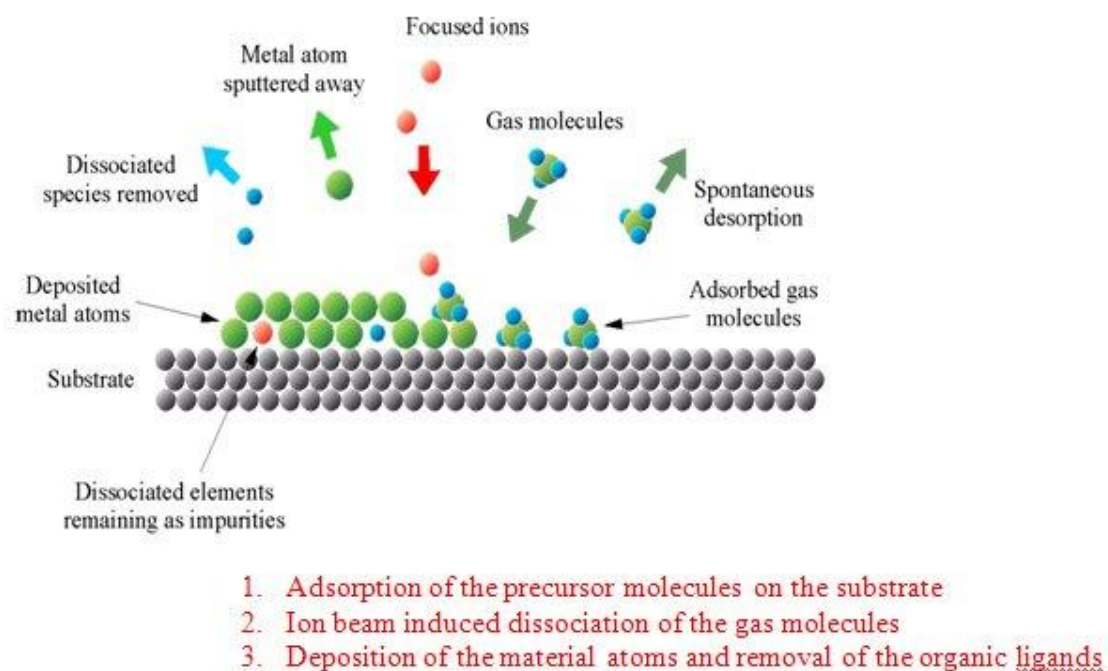
Figure 3.6 Schematic diagram of ion beam deposition [27]
