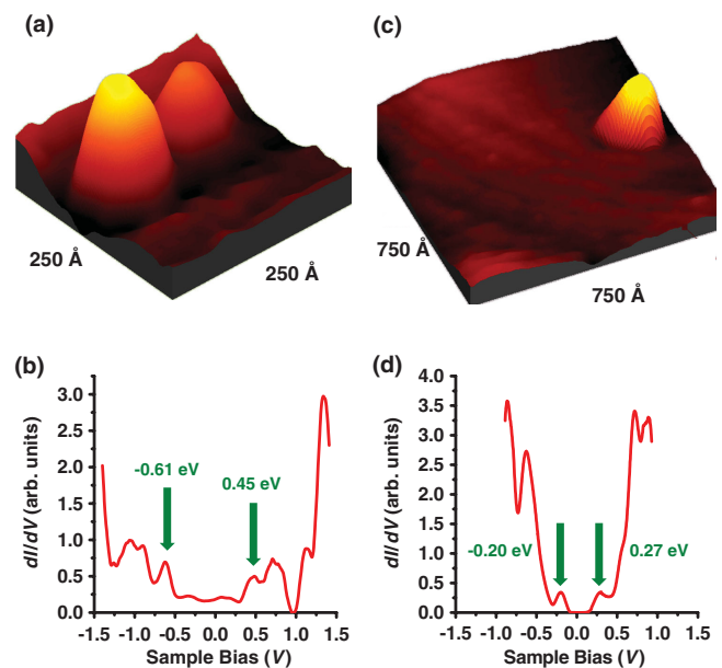
FIG. 4 (color). Scanning tunneling spectroscopy of individual GeTe nanoparticles. (a),(b) Topographic image (a) and plot of tunneling conductance vs sample bias (b) for amorphous GeTe nanoparticles. In-gap states and a band gap of \sim 1 \text{ eV} are observed. (c),(d) Topographic image (c) and plot of tunneling conductance (d) for crystallized, originally amorphous GeTe nanoparticles. No in-gap states and a band gap of \sim 0.4 \text{ eV} are observed.
