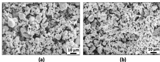
Figure 8. Scanning electron microscope images of YAG:Ce 3+ phosphor powder layer fabricated from (a) settling the powders (packing density <math>< 50\%</math>) and (b) a modified electrophoretic deposition (packing density = 69%). Adapted from Ref. 40.
