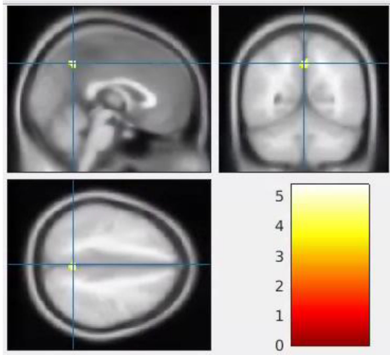
Fig. 2. Alteration of fractional amplitude of low-frequency fluctuation (fALFF) in the chemotherapy group from pre- (time point 1, TP1) to post-chemotherapy (time point 2, TP2). One cluster (indicated in yellow) in the left precuneus (0, -56, 44) shows a statistically significant decrease in fALFF from TP1 to TP2 ( p -corrected < 0.05 ). The blue crosshair indicates the cluster peak (0, -56, 44) in each plane. The color bar in the right lower panel indicates the scale of the t statistics for the within-group comparison of fALFF between TP1 and TP2.
