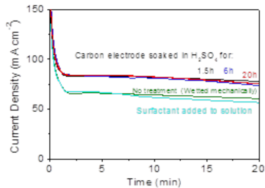
Figure 3. Impact of various treatments to improve solution wetting into the electrode. Potentiostatic discharge performance of Rayon 1200°C carbon felt at 0.55 V, gravity feed, compressed to 55% of original thickness, with coffee filter paper separator.
