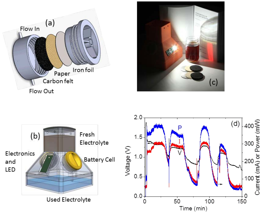
Figure 8. Prototype consumer product proof-of-concept. Schematics of (a) screw-cap cell sub-assembly and (b) complete product. (c) Image of product in operation, illuminating a textbook and the consumable electrolyte solution and cell components. (d) Performance of two cells in electrical series, connected to a LED driver circuit. Solution (200 mL) was collected and returned to the top electrolyte reservoir 4 times to achieve complete discharge. Cells contained Rayon 1200°C carbon felt pre-treated with H 2 SO 4 for 1.5 h and compressed to 55% of original thickness, and coffee filter paper separator (#3).
