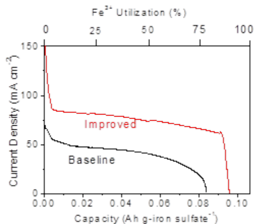
Figure 7. Improved potentiostatic discharge performance at 0.55 V with gravity flow, Rayon 1200°C carbon felt pre-treated with H 2 SO 4 for 6 h and compressed to 75% of original thickness, and coffee filter paper separator (#3). Baseline data from Ref. [6] is shown for comparison, with as-received Sigracet 10AA (+) electrode and office paper separator.
