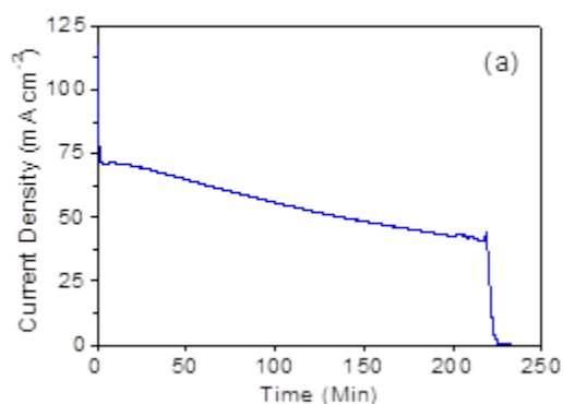
Figure 6. Use-case operation. (a) Long single potentiostatic discharge at 0.55V with 200 mL solution, gravity feed flow, coffee filter paper and Rayon 2000°C carbon felt.
