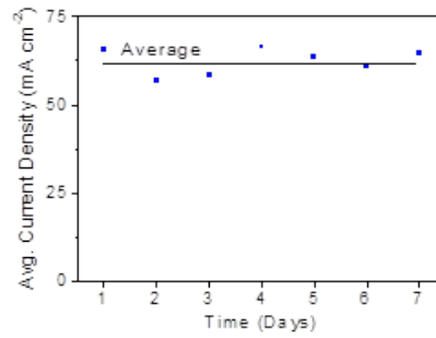
Figure 4. Carbon felt durability. One week of daily re-use of Rayon 1200°C carbon felt compressed to 75% of original thickness, 1 mL min -1 . Solution, filter paper, and iron steel foil were replaced each day.
