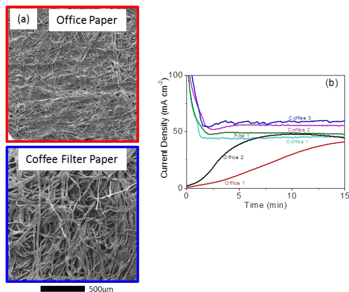
Figure 5. Performance of various paper separators. (a) SEM images of office and coffee filter papers. (b) Potentiostatic discharge performance at 0.55 V, 1 mL min -1 , with Rayon 1200°C carbon felt compressed to 85% of original thickness.
