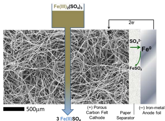
Figure 1. Schematic of the all-iron flow cell. The horizontal axis in the image is to scale. The iron sulfate solution is introduced by gravity feed from an inlet reservoir, and flows through the entire thickness of the porous carbon cathode.
