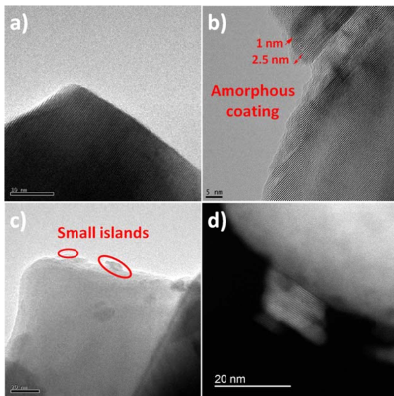
Figure 5.7 TEM and STEM photographs of LNMO and NALNMO, (a) TEM of LNMO, (b) and (c) TEM of NALNMO, (d) STEM of NALNMO.
