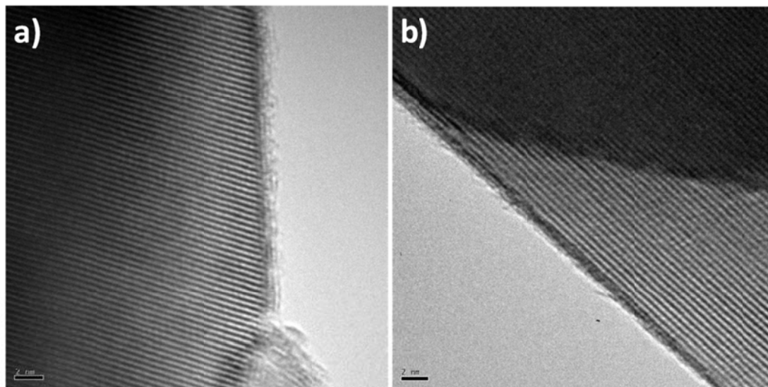
Figure 5.8 TEM photographs of pristine NALNMO, prepared from carbonate method.
