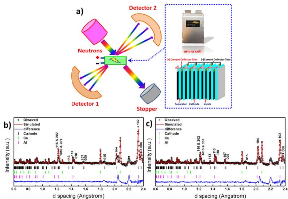
Figure 4.1 (a) schematic of the operando neutron diffraction study and the pouch cell. (b) refined diffraction pattern of HLR / Si cell and (c) LLR / Si cell at the open circuit potential state.
