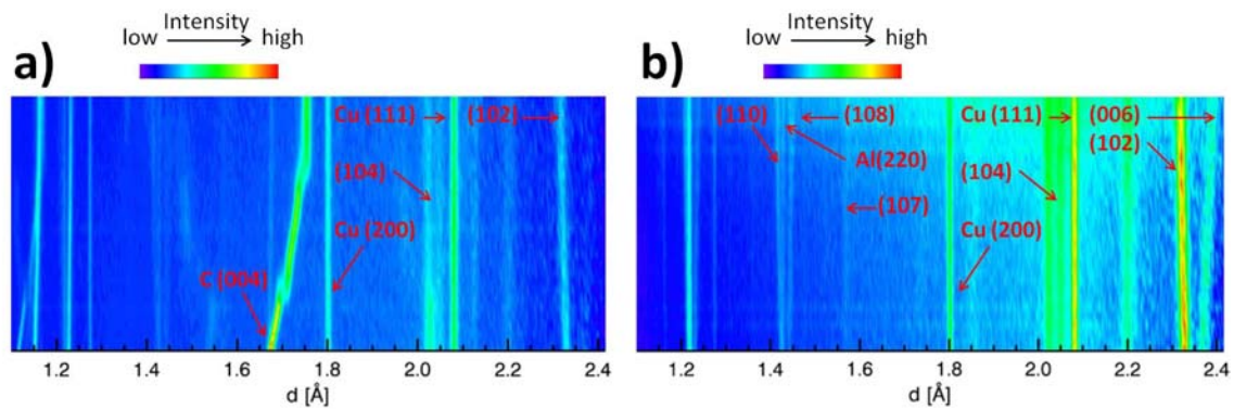
Figure 4.2 Neutron diffraction contour plots of (a) LR / graphite cell and (b) for the HLR / Si cell during charge (5 hours charging data).
