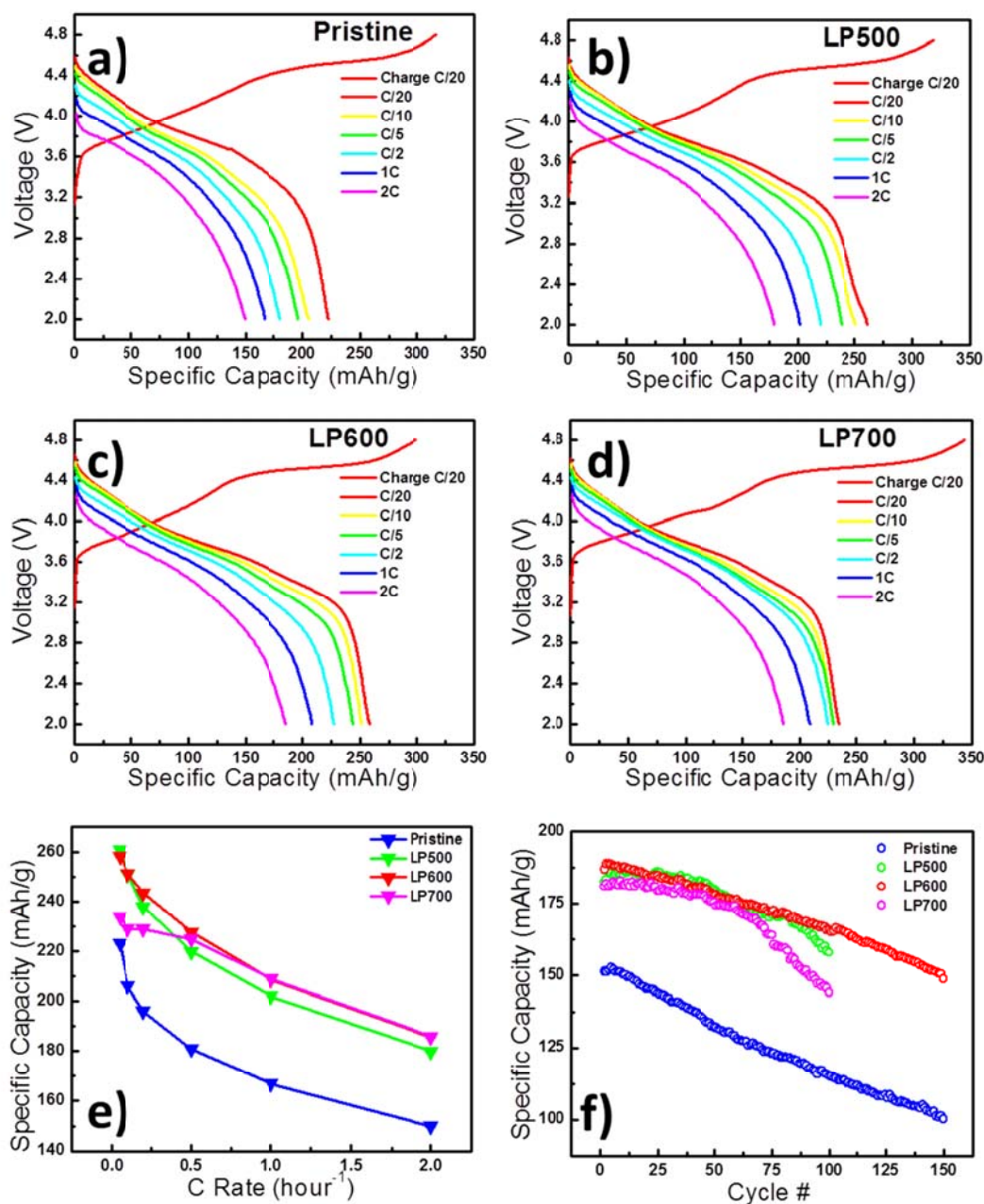
Figure 6.3 Comparison of electrochemical performances between LNMO and LPLNMOs: (a)-(d) voltage profiles under different current density; (e) discharge capacity under different current density; and (f) comparison of capacity upon cycling, the voltage range is 2.0–4.8 V at 1 C = 250 mA g -1 .
