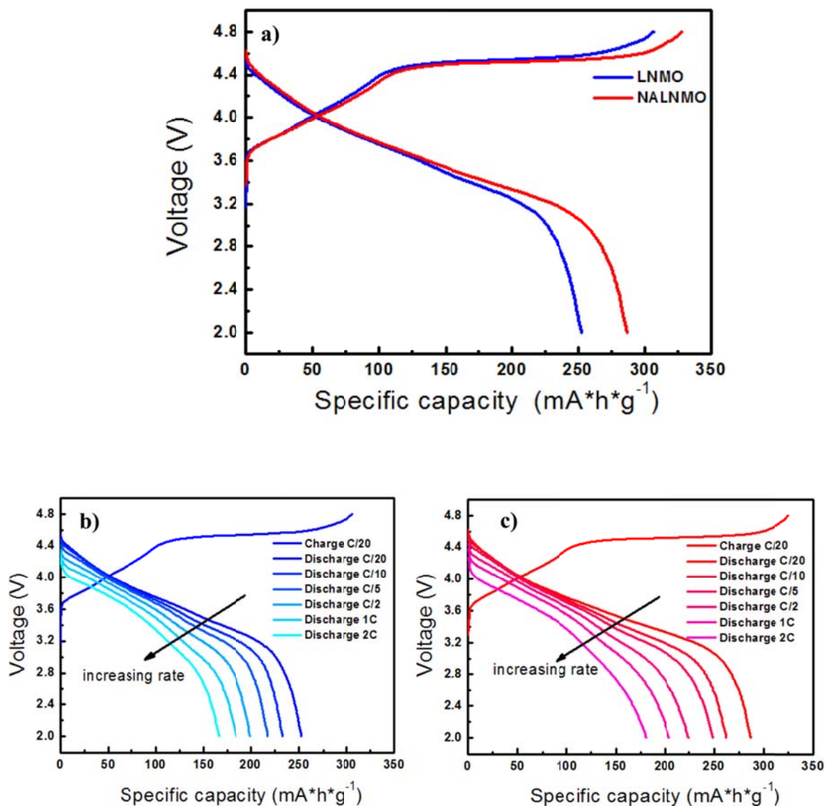
Figure 5.4 Comparison of electrochemical performances between LNMO and NALNMO. (a) first cycle charge/ discharge voltage profile, (b) voltage profile of LNMO under different current density, (c) voltage profile of NALNMO under different current density. Voltage range is 2.0 - 4.8 V at 1\text{C} = 250\text{ mA g}^{-1} .
