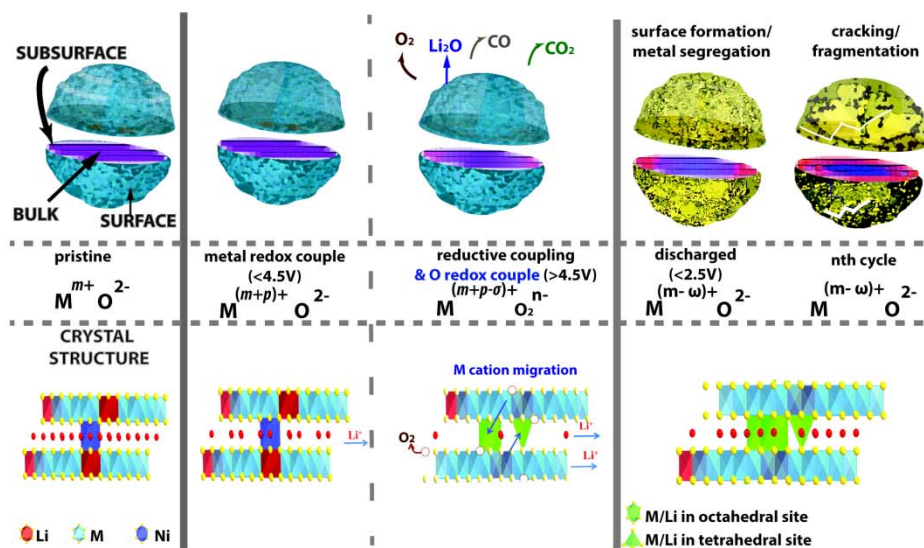
Figure 1.5 Schematic diagram of the changes that occur during electrochemical cycling that occurs within the surface and the crystal structure. The middle represents the changes in the redox for the cation and anions that participate in the charging compensation mechanism.
