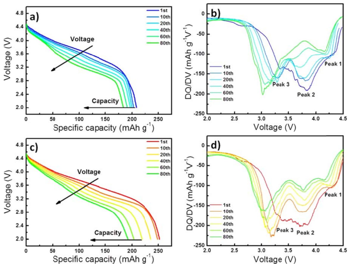
Figure 5.6 Discharge and corresponding dQ/dV profiles of (a) & (b) LNMO and (c) & (d) NALNMO, over the course of 80 cycles.
