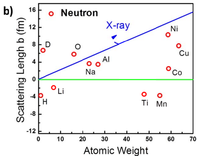
Figure 2.2 (a) The schematic of X-ray and neutron interact with atoms. (b) Comparison of neutron and X-ray atomic scattering powers.
