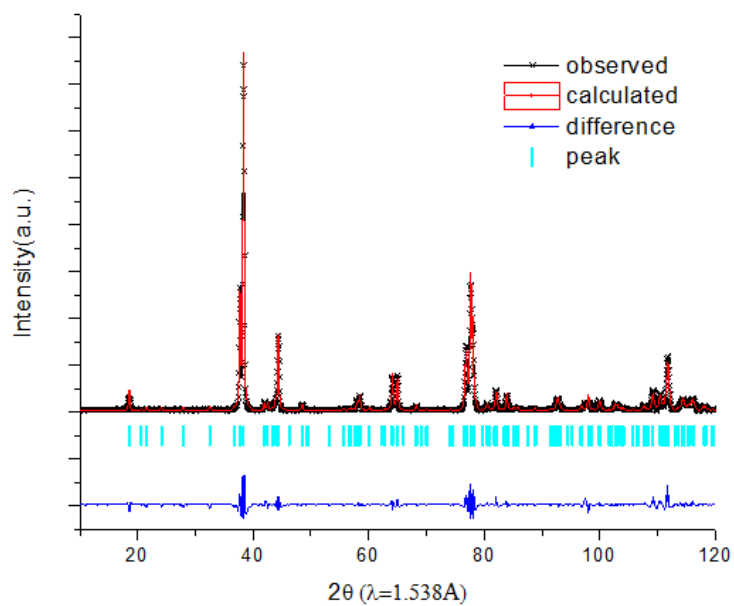
Figure 3.6 Ex-situ neutron diffraction patterns and profile matching with C/2m space group result of pristine \text{Li}[\text{Li}_{0.2}\text{Ni}_{0.2}\text{Mn}_{0.6}]\text{O}_2 .
