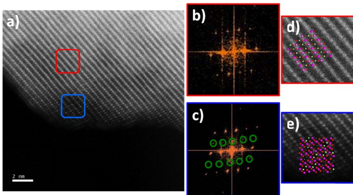
Figure 5.10 High-resolution STEM images of NALNMO, (a) NALNMO, (d) bulk region and (e) surface region. The fast Fourier transform FFT, (b) bulk region and (c) surface region. (The insets crystal structure in (d) and (e), green: Li, red: O, purple: transition metal)
