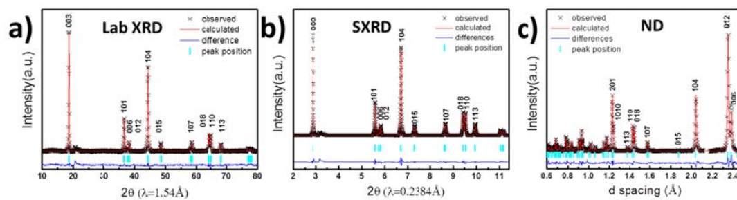
Figure 2.5 The refinement of \text{Li}_{1.13}\text{Ni}_{0.3}\text{Mn}_{0.567}\text{O}_2 (a) using in house lab XRD; (b) using APS synchrotron XRD; (c) using neutron diffraction.
