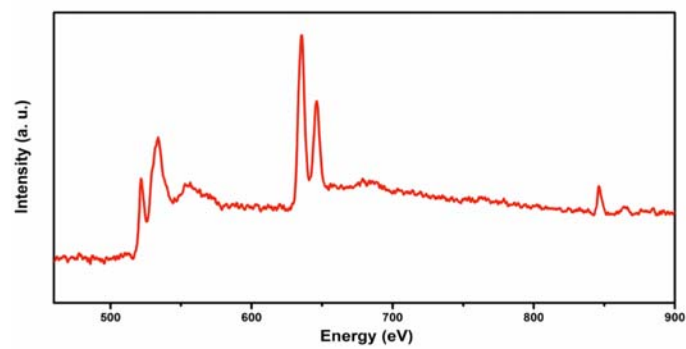
Figure 5.9 EELS spectrum of crystalline nano-islands at the surface of NALNMO.
