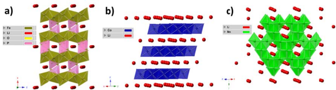
Figure 1.2 Schematics of crystal structures of a) \text{LiFePO}_4 , b) \text{LiCoO}_2 , and c) \text{LiMn}_2\text{O}_4 .
