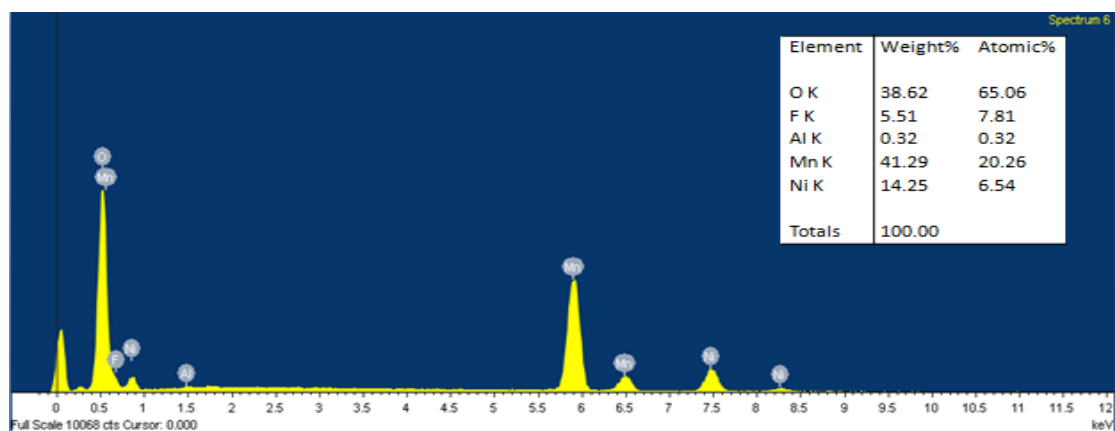
Figure 5.2 EDS spectrum of NALNMO starting material.
