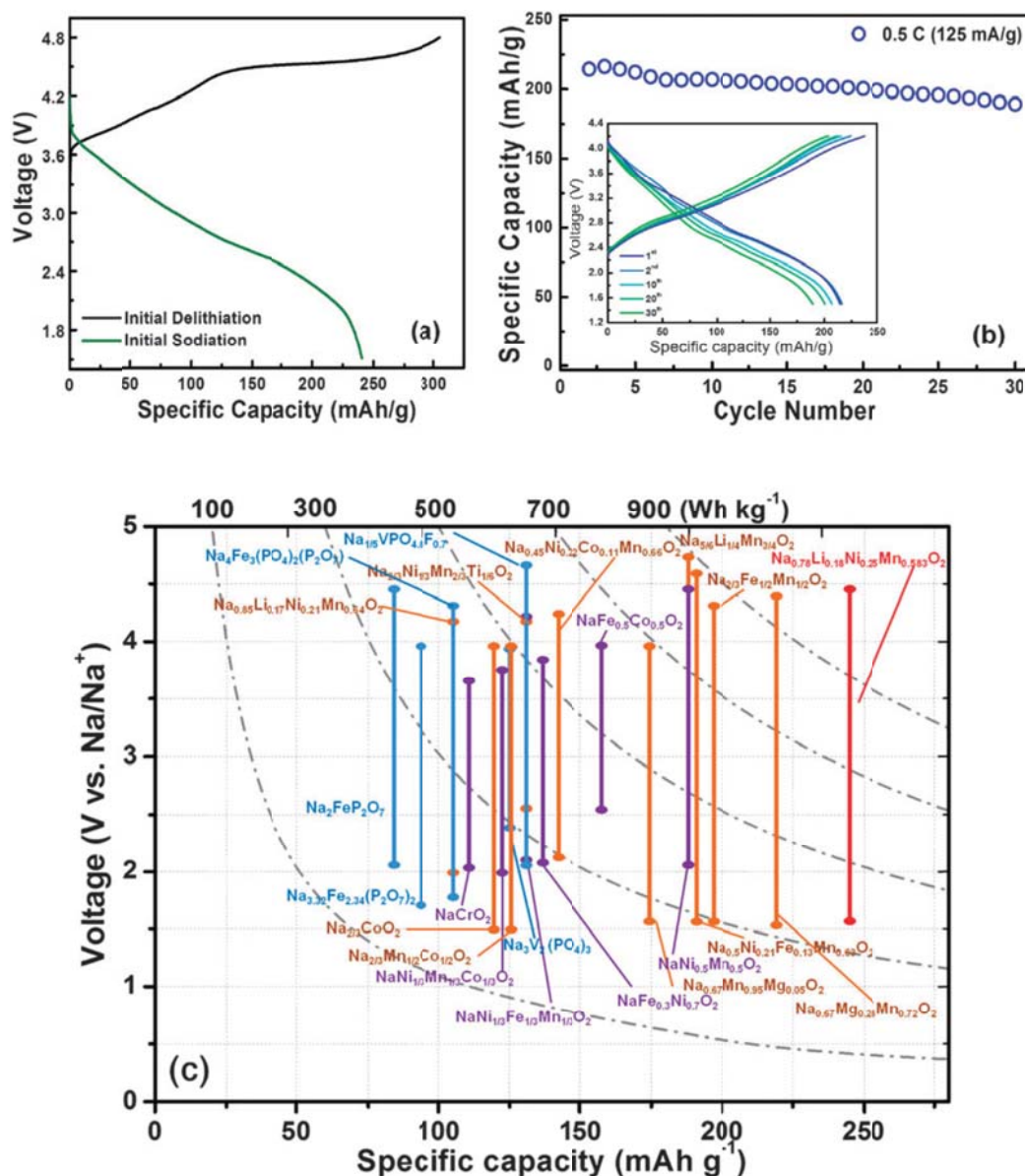
Figure 7.2 (a) Electrochemical profiles of initial delithiation and initial sodiation for \text{Na}_{0.78}\text{Li}_{0.18}\text{Ni}_{0.25}\text{Mn}_{0.583}\text{O}_w in half cell. (b) Cycling performance for \text{Na}_{0.78}\text{Li}_{0.18}\text{Ni}_{0.25}\text{Mn}_{0.583}\text{O}_w with 125 mA g -1 current density. Inset is the corresponding electrochemical profile of \text{Na}_{0.78}\text{Li}_{0.18}\text{Ni}_{0.25}\text{Mn}_{0.583}\text{O}_w during the 1 st , 2 nd , 10 th , 20 th , 30 th cycles in Na-ion batteries. (c) Comparison of reversible capacities for the intercalation-based Na cathodes. 199, 206, 222-241
