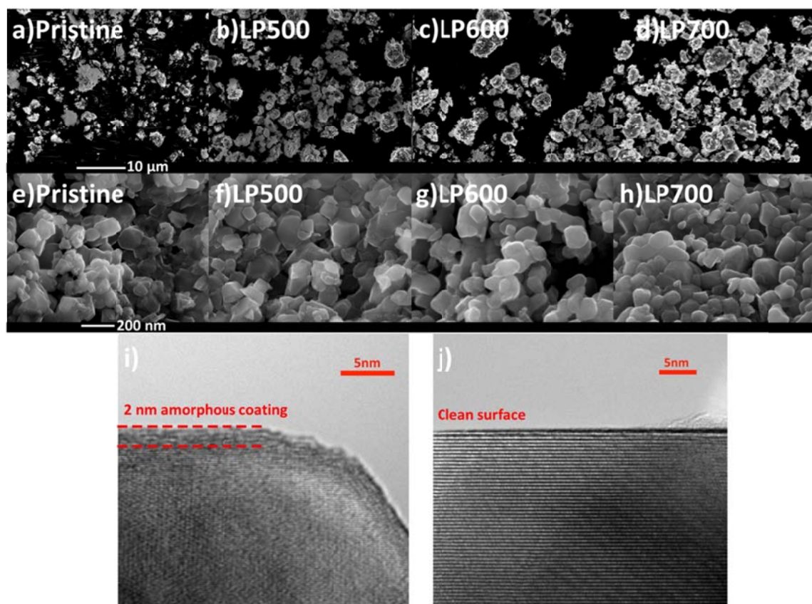
Figure 6.1 SEM images: (a)-(h). TEM images of LP600: (i) particles with coating and (j) particles that were surface modified but still were not coated.
