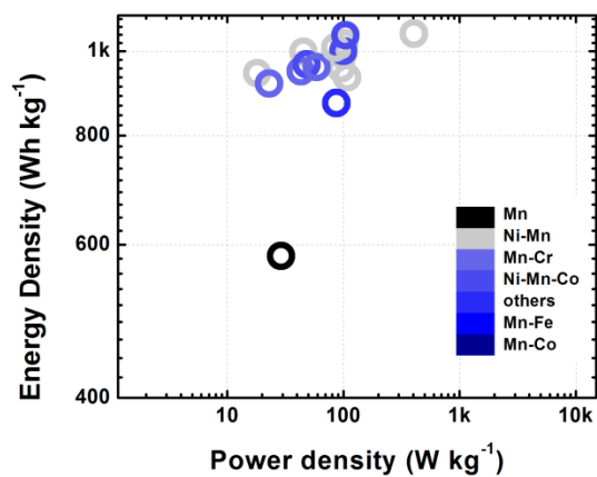
Figure 1.4 Ragone plot at the material level exhibiting the highest first discharge capacity for each year from Figure 1.3 (dashed black line).
