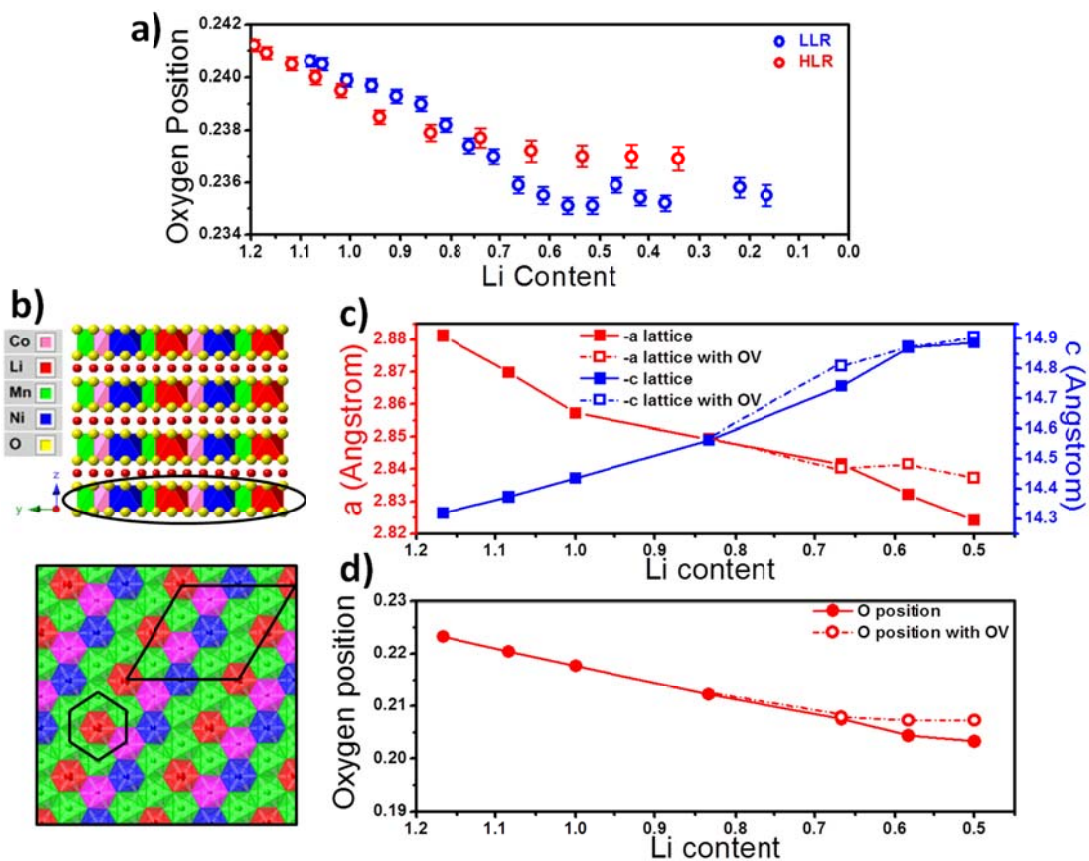
Figure 4.5 (a) oxygen position from refinement results, (b) the cation ordering in TM layer used for DFT calculations, (c) DFT results of the evolution of the lattice parameters and (d) oxygen position with and without oxygen vacancy.
