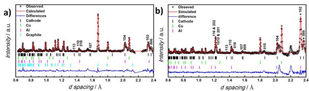
Figure 4.3 Refined diffraction pattern of (a) LR / graphite cell and (b) HLR / Si cell at the open circuit potential state.
