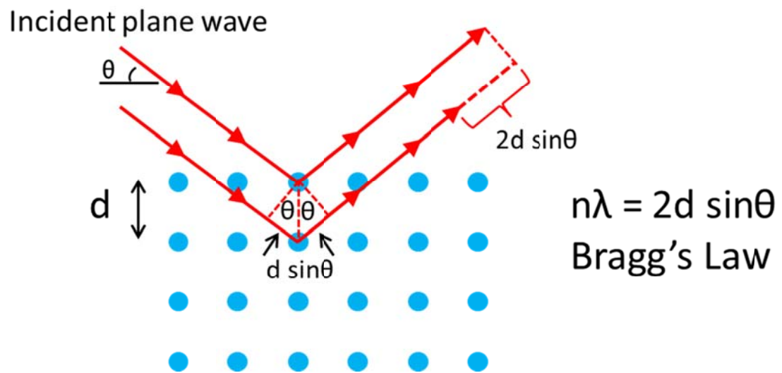
Figure 2.1 Two dimensional illustration of Bragg's law.
