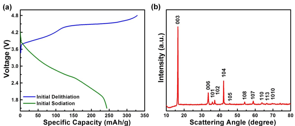
Figure 7.8 (a) The electrochemical profile for \text{Li}_{1.167}\text{Ni}_{0.166}\text{Mn}_{0.5}\text{Co}_{0.166}\text{O}_2 during initial delithiation and initial sodiation. (b) XRD for as-synthesized \text{NaLi}_{0.067}\text{Co}_{0.267}\text{Ni}_{0.267}\text{Mn}_{0.4}\text{O}_2 .
