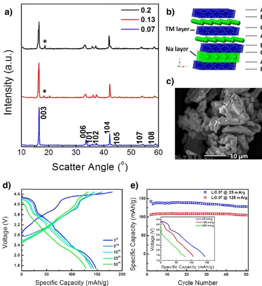
Figure 8.1 (a) Powder XRD for \text{NaLi}_x\text{Ni}_{1/3-x}\text{Mn}_{1/3+x}\text{Co}_{1/3-x}\text{O}_2 ( x = 0.07, 0.13 , and 0.2 ). (* is the peak from impurity phase) (b) Schematic of the typical O3 structure. (c) SEM of the \text{NaLi}_{0.07}\text{Ni}_{0.26}\text{Mn}_{0.4}\text{Co}_{0.26}\text{O}_2 . (d) Electrochemical profiles of \text{NaLi}_{0.07}\text{Ni}_{0.26}\text{Mn}_{0.4}\text{Co}_{0.26}\text{O}_2 in half cell. (e) Cycling performance for \text{NaLi}_{0.07}\text{Ni}_{0.26}\text{Mn}_{0.4}\text{Co}_{0.26}\text{O}_2 at different current densities. Inset is the electrochemical profiles of \text{NaLi}_{0.07}\text{Ni}_{0.26}\text{Mn}_{0.4}\text{Co}_{0.26}\text{O}_2 at 25 \text{ mA g}^{-1} , 125 \text{ mA g}^{-1} , and 500 \text{ mA g}^{-1} current density.
