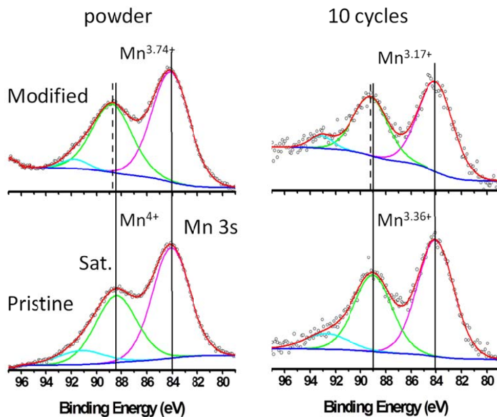
Figure 5.13 XPS Mn 3s regions of LNMO and NALNMO pristine and cycled electrode materials.
