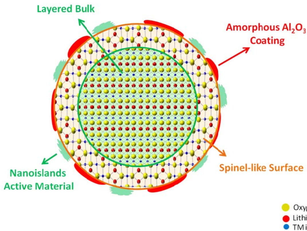
Figure 5.14 Schematic of proposed structure model of NALNMO (not draw to scale).
