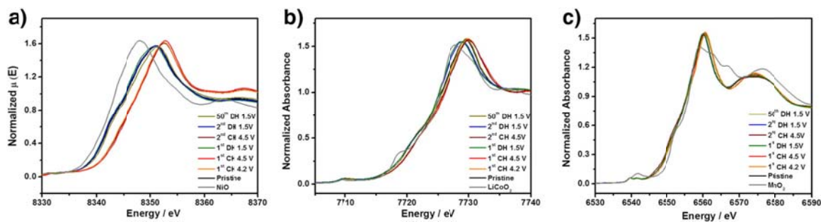
Figure 8.3 Ex-situ XAS analysis for \text{NaLi}_{0.07}\text{Ni}_{0.26}\text{Mn}_{0.4}\text{Co}_{0.26}\text{O}_2 at different states. XANES spectra for (a) Ni, (b) Co and (c) Mn K-edge respectively.
