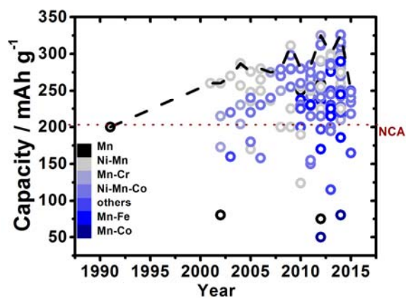
Figure 1.3 Evolution of the discharge capacity by years.
