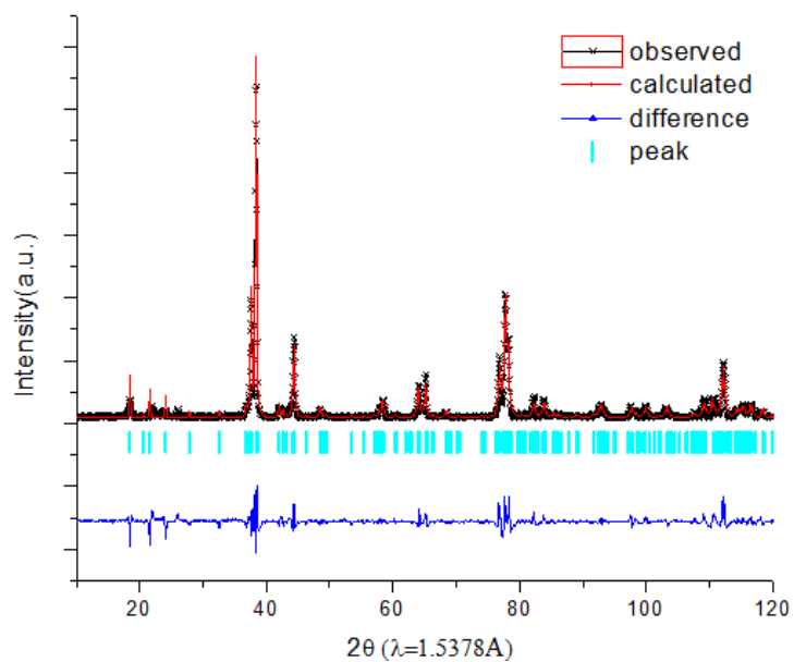
Figure 3.8 Ex-situ neutron diffraction patterns and profile matching with C/2m space group result of chemically delithiated sample \text{Li}_{0.4}\text{Ni}_{0.2}\text{Mn}_{0.6}\text{O}_{1.8} .
