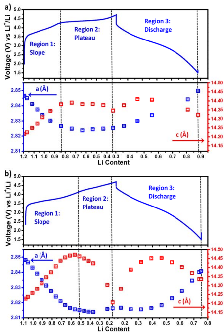
Figure 4.4 Electrochemical charge/discharge profile with corresponding lattice parameters at different states of delithiation/lithiation for (a) HLR and (b) LLR.
