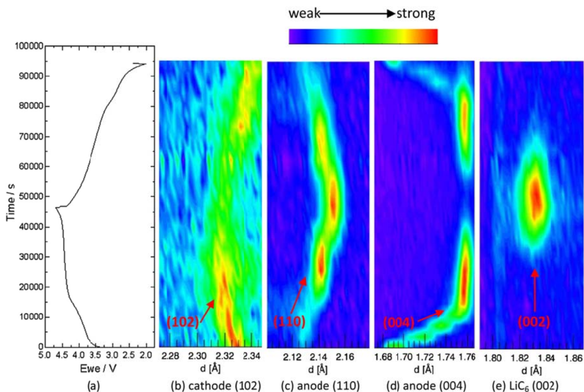
Figure 3.3 (a) 1 st cycle charge/discharge curve of \text{Li}[\text{Li}_{0.2}\text{Ni}_{0.18}\text{Mn}_{0.53}\text{Co}_{0.1}]\text{O}_2 and surface contour plots of (b) \text{Li}[\text{Li}_{0.2}\text{Ni}_{0.18}\text{Mn}_{0.53}\text{Co}_{0.1}]\text{O}_2 (102); (c) \text{Li}_x\text{C}_6 (110); (d) \text{Li}_x\text{C}_6 (004); (e) \text{LiC}_6 (002) Neutron Diffractions.
