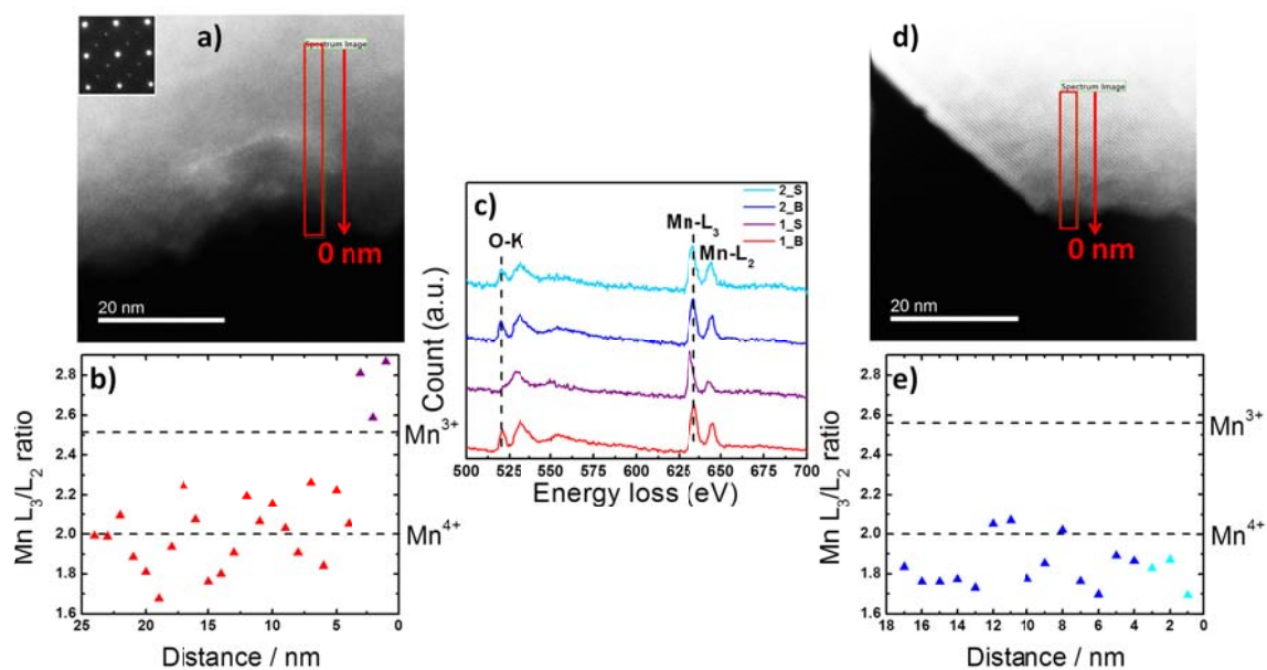
Figure 5.11 STEM images of NALNMO with step scan of Mn EELS L edge and O EELS K edge. (a) STEM of NALNMO with C2/m domain, (b) corresponding Mn L 3 /L 2 ratio, (c) representative EELS spectra of the Mn L edge and O K edge from the surface and bulk of NALNMO with different domains, (1 is C2/m domain particle, 2 is R \bar{3} m domain particle, S represent surface, B represent bulk), (d) STEM of NALNMO with R \bar{3} m domain, and (e) corresponding Mn L 3 /L 2 ratio.
