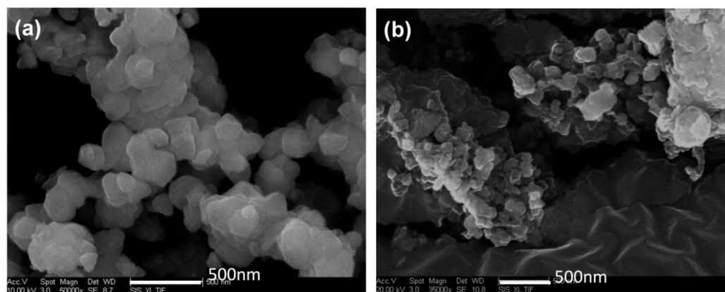
Figure 7.3 SEM images for (a) as-synthesized \text{Li}_{1.167}\text{Ni}_{0.25}\text{Mn}_{0.583}\text{O}_2 and (b) \text{Na}_{0.78}\text{Li}_{0.18}\text{Ni}_{0.25}\text{Mn}_{0.583}\text{O}_w .
