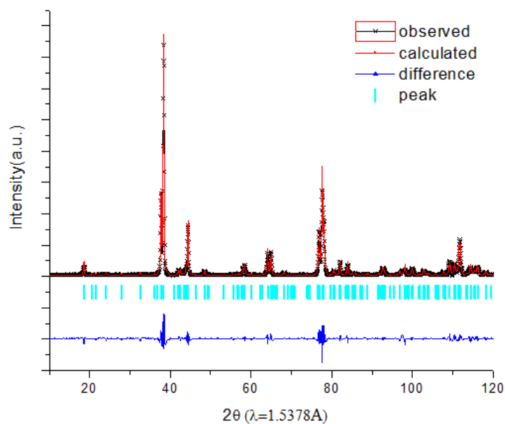
Figure 3.7 Ex-situ neutron diffraction patterns and profile matching with P3_112 space group result of pristine \text{Li}[\text{Li}_{0.2}\text{Ni}_{0.2}\text{Mn}_{0.6}]\text{O}_2 .
