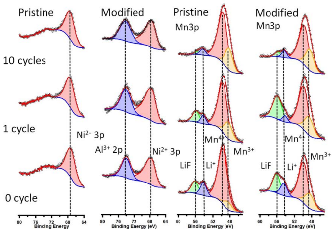
Figure 5.12 Ni 3p and Mn 3p core level X-ray photoelectron spectra of LNMO and NALNMO at various stages of cycling.
