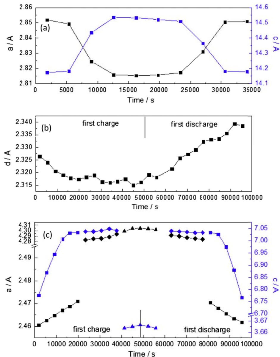
Figure 3.4 (a) Cathode \text{Li}[\text{Ni}_{1/3}\text{Mn}_{1/3}\text{Co}_{1/3}]\text{O}_2 lattice parameters change during 1 st cycle, black is the a -parameter, blue is the c -parameter; (b) \text{Li}[\text{Li}_{0.2}\text{Ni}_{0.18}\text{Mn}_{0.53}\text{Co}_{0.1}]\text{O}_2 (102) d -spacing change during 1 st cycle; (c) anode graphite lattice parameter change during 1 st cycle, black is the a -parameter, blue is the c -parameter, the square is the \text{Li}_x\text{C}_6 phase, the diamond is the \text{LiC}_{12} phase, the triangle is the \text{LiC}_6 phase.
