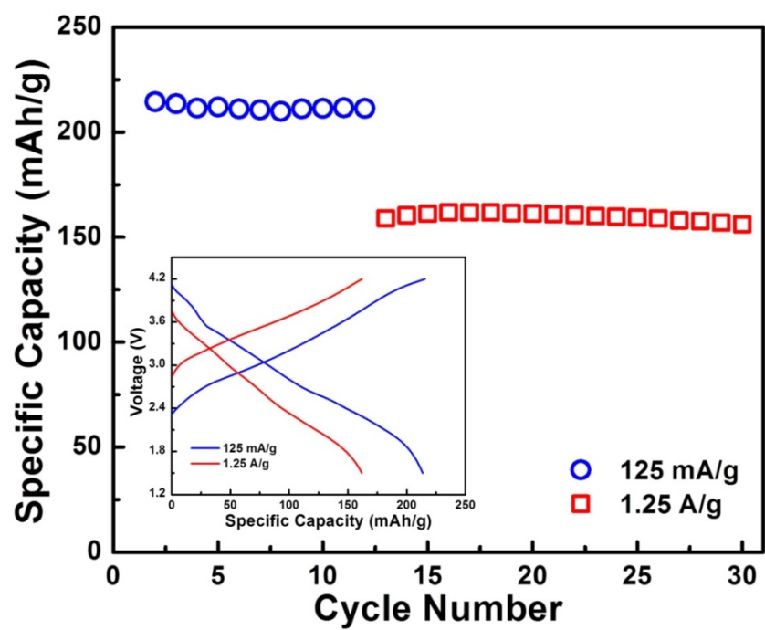
Figure 7.4 Rate performance for \text{Na}_{0.78}\text{Li}_{0.18}\text{Ni}_{0.25}\text{Mn}_{0.583}\text{O}_w .
