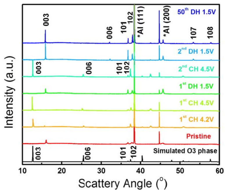
Figure 8.2 Ex-situ SXR D for \text{NaLi}_{0.07}\text{Ni}_{0.26}\text{Mn}_{0.4}\text{Co}_{0.26}\text{O}_2 at different states.
