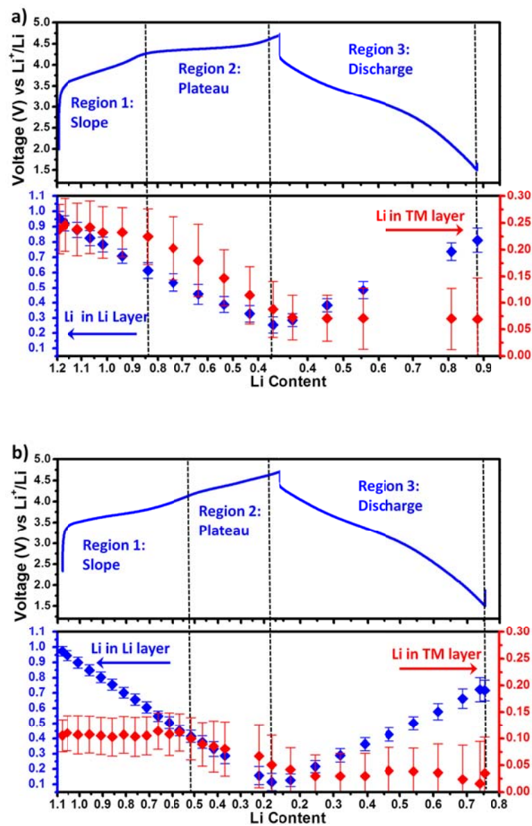
Figure 4.6 Electrochemical charge/discharge profile with corresponding lithium occupancy at different states of delithiation/lithiation for (a) HLR and (b) LLR.
