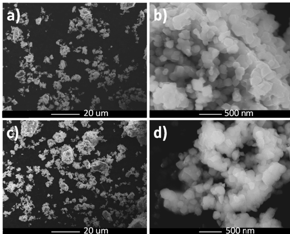
Figure 5.1 SEM images: (a) and (b) are LNMO, (c) and (d) are NALNMO.
