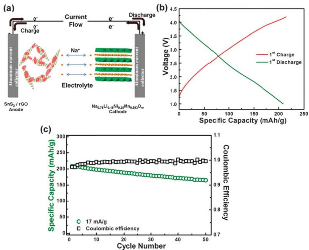
Figure 7.7 (a) Schematic of Na full cell. (b) The electrochemical profile at 1 st cycle and (c) cycling performance for the Na full cell.
