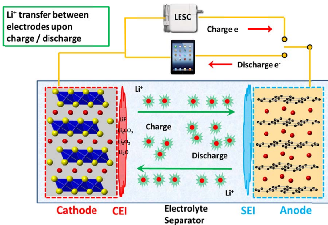
Figure 1.1 Schematic of a rechargeable Li-ion battery.
