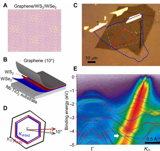
Fig. 1. Moiré superlattices of graphene/ WS_2/WSe_2 . (A) Schematic atomic arrangement of an aligned WS_2/WSe_2 moiré superlattice with a graphene layer, where WS_2 , WSe_2 , and graphene layers are in red, blue, and gray, respectively. (B and C) Schematics (B) and optical micrograph (C) of a moiré superlattice sample on a Nb:TiO 2 substrate, where WS_2 , WSe_2 , and graphene are represented by red, blue, and gray colors, respectively. (D) Schematic of Brillouin zones of WS_2 (red), WSe_2 (blue), and graphene (gray). (E) ARPES spectra taken along \Gamma - K_G , with overlaid density functional theory (DFT) calculations of the band structures for individual monolayer graphene (gray), WS_2 (red), and WSe_2 (blue). The white arrow indicates hybridization between the graphene and TMD bands.
