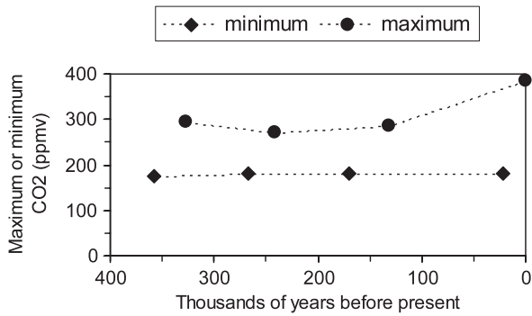
Figure 7. Minimum and maximum atmospheric CO 2 concentrations during ice ages and interglacial periods, respectively, over the last 400 000 years.
