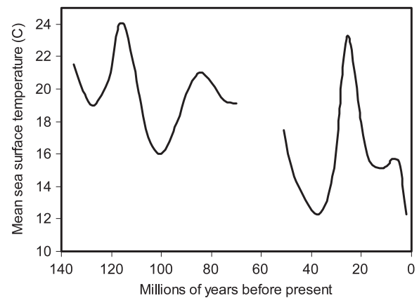
Figure 3. Mean sea surface temperature in the northern mid-latitudes (after Budyko 1977). The gap about 65 millions years before present coincides with the Cretaceous–Tertiary (K–T) boundary and the meteoric impact theorized to have occurred then.
