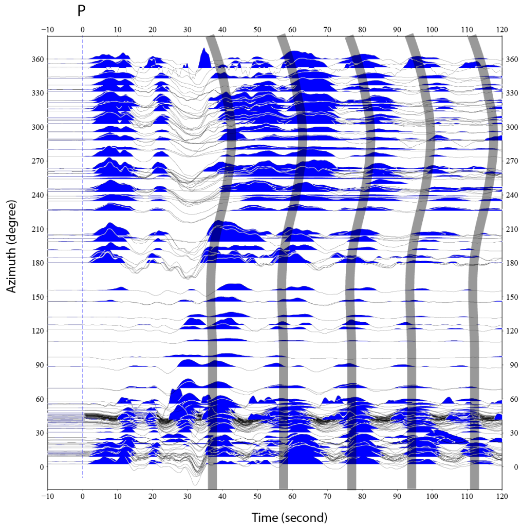
Figure S2. Azimuthal plot of the teleseismic P waveforms for the 3 May 2006 Tonga event, aligned on the P arrivals. Grey shadows indicate strong multiple water phase vibrations.
