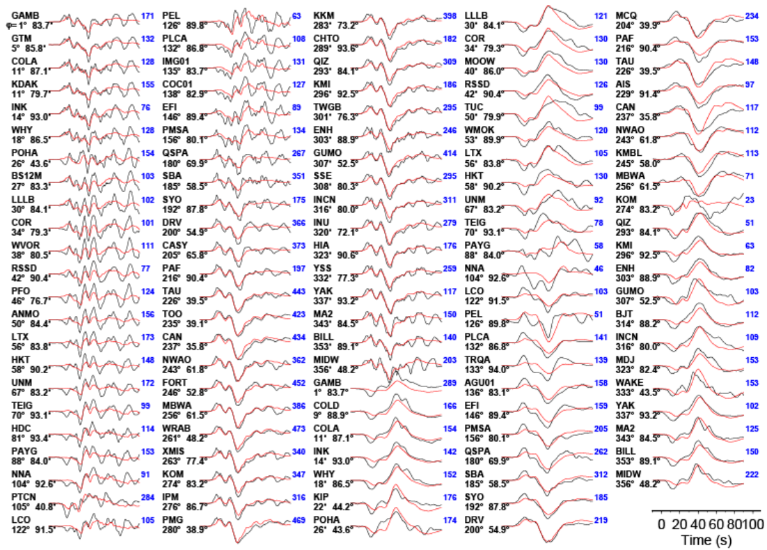
Figure S4. Observed (black) and predicted (red) teleseismic P and SH waveforms for the 3 May 2006 Tonga event for the joint inversion of teleseismic body waves and local static offsets for the steeply dipping fault in Figure 8b.
