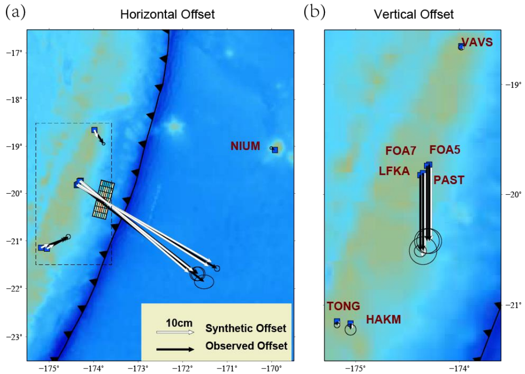
Figure S5. Locations of local GPS campaign stations (blue squares) that provide horizontal (black vectors in (a)) and vertical (black vectors in (b)) co-seismic offsets, within which (b) is a zoomed area of the dashed rectangle in (a), for the 3 May 2006 Tonga event. Their uncertainties (95% probability) are indicated by black ellipses. Predicted displacements for the steeply dipping fault plane model in Figure 8a are shown by red vectors for horizontal motions (a) and for vertical static offsets (b). The fits are comparable to those for the shallowly dipping fault plane shown in Figure 10.
