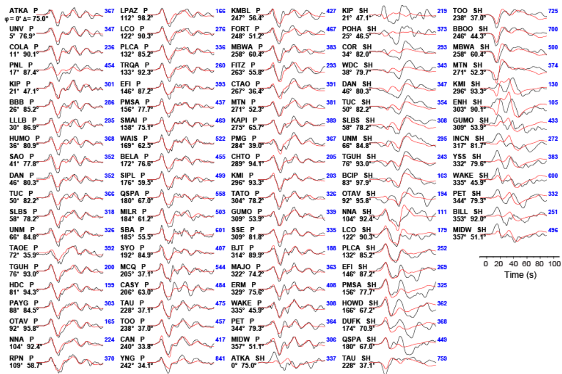
Figure S7. Observed (black) and predicted (red) teleseismic P and SH waveforms for the 19 March 2009 Tonga event for the inversion of teleseismic body waves for the eastward dipping fault shown in Figure 14.
