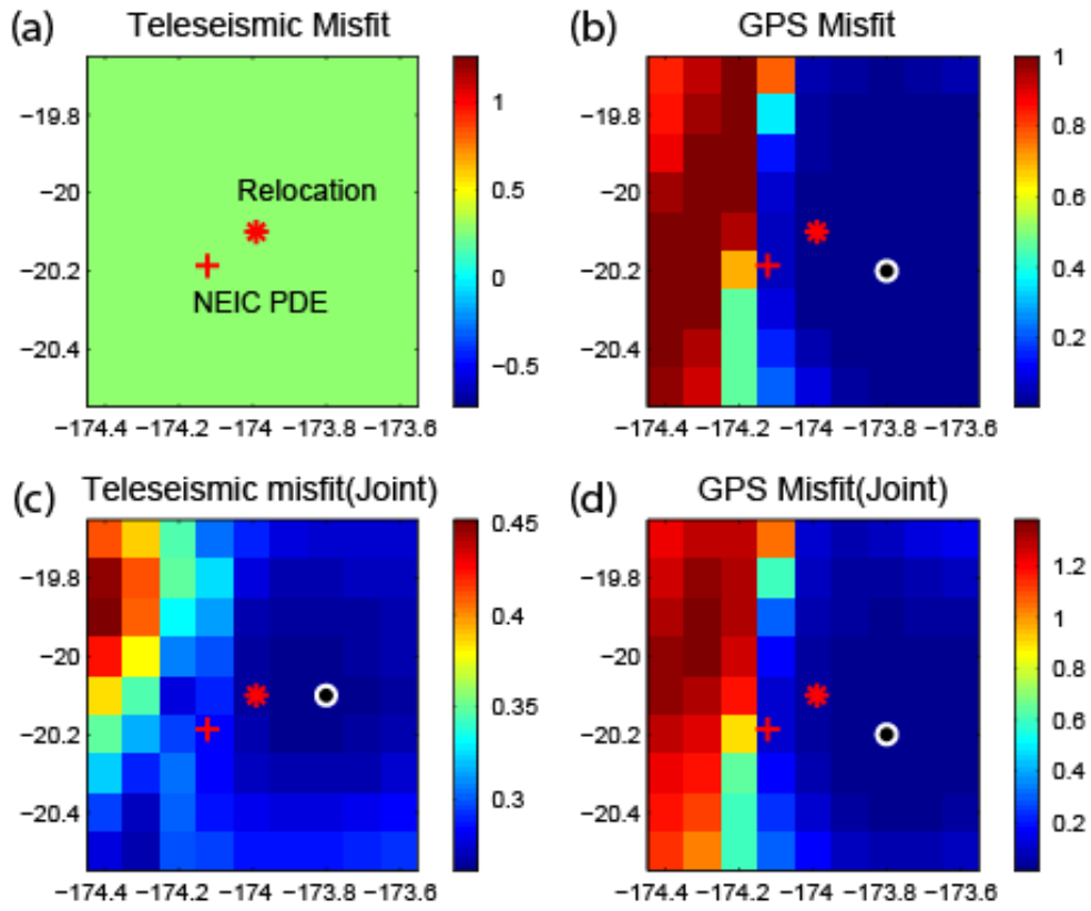
Figure 7. Residual waveform misfit distributions for a 65 km deep grid of hypocentral locations for the 3 May 2006 Tonga mainshock for the steeply dipping fault plane showing (a) teleseismic body wave inversion misfits (b) local GPS static offset inversion misfits (station locations are shown in Figure 10) (c) teleseismic body wave misfits for joint inversion of teleseismic and GPS data and (d) GPS static offset misfits for joint inversion of teleseismic and GPS data. White circles indicate locations that give minimum residuals for the separate data sets in the joint inversions, relative to the USGS/NEIC location (red plus signs), and the locally relocated hypocenter (red asterisks).
