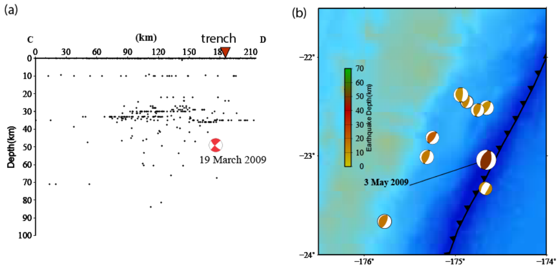
Figure S6. (a) Cross-section view of aftershocks from the USGS-NEIC catalog for the 19 March 2009 Tonga event along profile CD in Figure 2. The scatter in the unrelocated locations is too large to confidently identify the megathrust, but the mainshock hypocenter clearly plots below the distributed aftershocks and they are concentrated to the NW. (b) GCMT focal mechanisms of the mainshock and aftershocks in the following 3 months. The latter events range in magnitude from 5.0 to 5.5. All but one of the aftershocks has a shallow-dipping thrust fault mechanism. The thrust fault aftershocks have GCMT depths ranging from 12 to 22 km, and the normal faulting event below the trench has a depth of 13 km. It appears that megathrust faulting was induced by the deep intraplate compressional earthquake.
