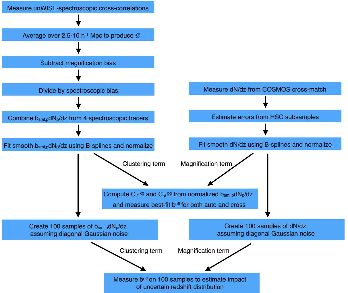
Figure 3. An outline of the steps required to interpret the angular clustering of the unWISE samples: estimate the redshift distribution, fit a linear bias to C_\ell^{kg} and C_\ell^{gg} , and estimate the impact of uncertainty in the redshift distribution on the fitted biases.
