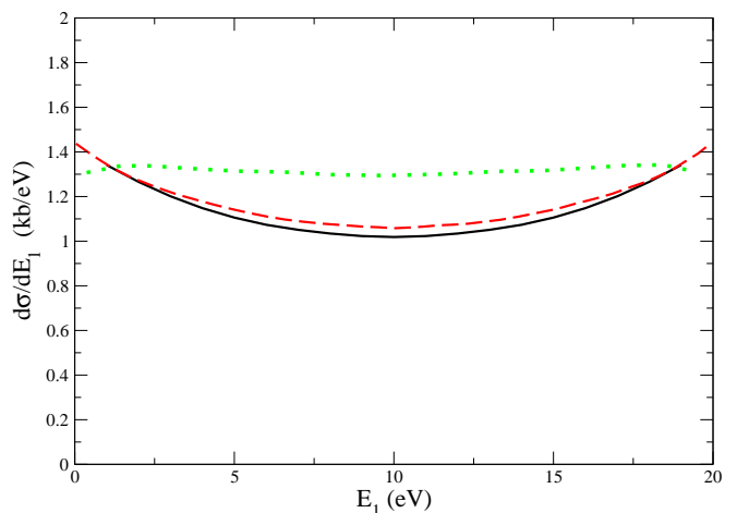
FIG. 4: (Color online) Single differential cross section (SDCS) results for DPI of beryllium at 20 eV excess photon energy. Solid curve: present results; dashed curve: results of Colgan and Pindzola [10]; dotted curve: HRM-SOW results of Citrini, et. al. [11].
