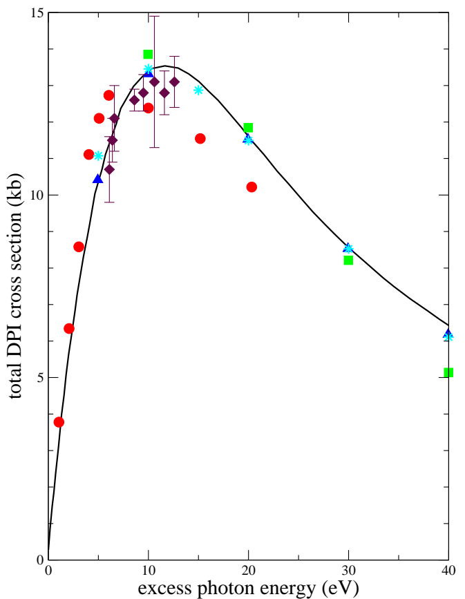
FIG. 3: (Color online) Total DPI cross section from beryllium at various energies. Stars: present results, solid curve: polynomial fit to RMPS calculation [13] of Griffin, et. al. , solid circles: CCC results of Kheifets and Bray [9], solid squares: TDCC results of Colgan and Pindzola [10], solid triangles: B -spline results of Laulan and Bachau [12], solid diamonds with error bars: experimental measurements of Wehlitz, et. al. [16]. 1 \text{ kb} = 10^{-21} \text{ cm}^2 .
