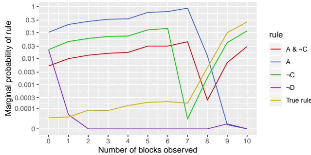
Figure 2: Rule probabilities by number of observations. In the near condition (left), the true rule was most probable under the model, although other rules which explained 9/10 blocks were also assigned non-negligible probabilities. In the distant condition (right), the true rule's final probability was near 1.
