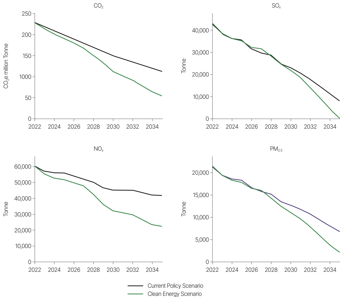
Figure 13. Electricity Sector Emissions of CO 2 , SO x , NO x and PM 2.5 Through 2035
