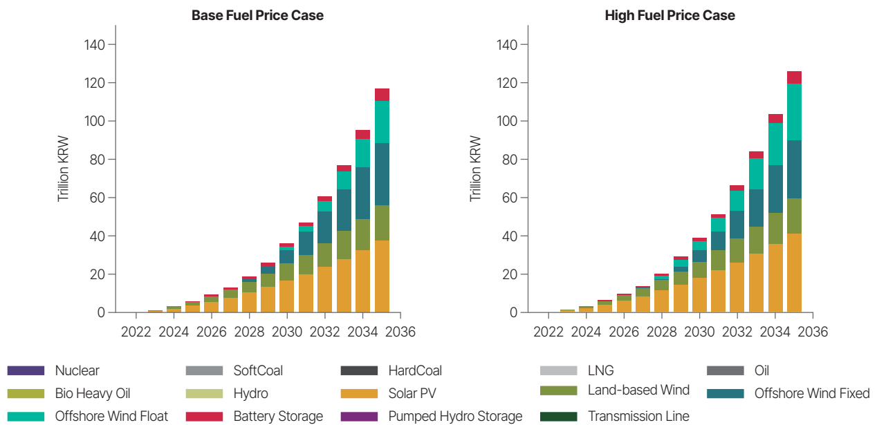
Figure 25. Cumulative New Capital Investment in Generation and Transmission, Clean Energy Scenario with Base vs. High Fuel Price Cases
