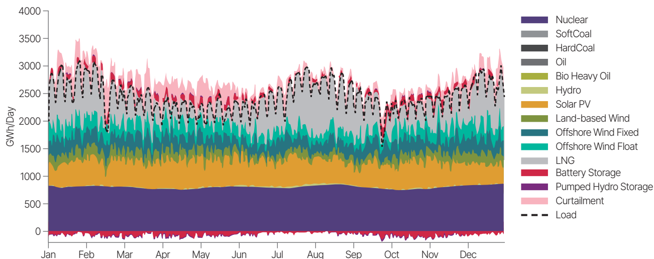
Figure 21. Daily National System Dispatch Averaged Over 7 Weather Years in the Clean Energy Scenario in 2035
