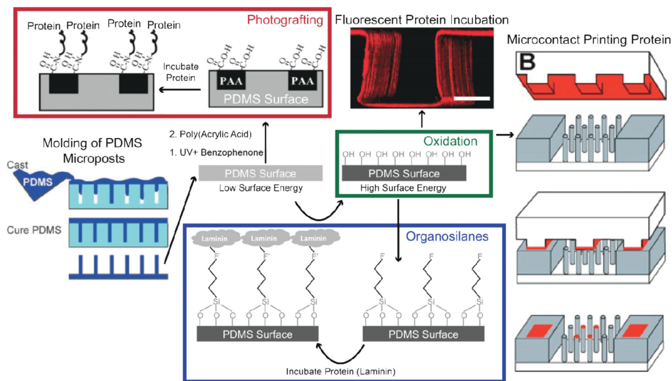
Figure 7. Different methods to functionalized PDMS surfaces
