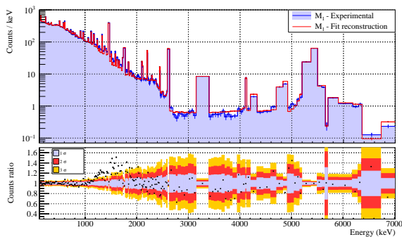
Fig. 13 CUORE-0 \mathcal{M}_1 compared to the reconstruction predicted by the fit without the 2\nu\beta\beta source.
