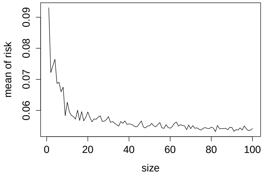
Figure 5.2: the Mean of Portfolio Risk
