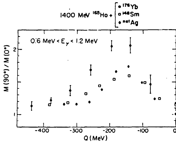
Figure 11. \gamma -ray anisotropy as a function of Q value for the reactions 1400 \text{ MeV } ^{165}\text{Ho} + ^{\text{nat}}\text{Ag} , ^{148}\text{Sm} and ^{176}\text{Yb} , for heavy ions detected near the grazing angle. Error bars for the three systems are similar and are shown only for ^{165}\text{Ho} + ^{176}\text{Yb} 20 .
