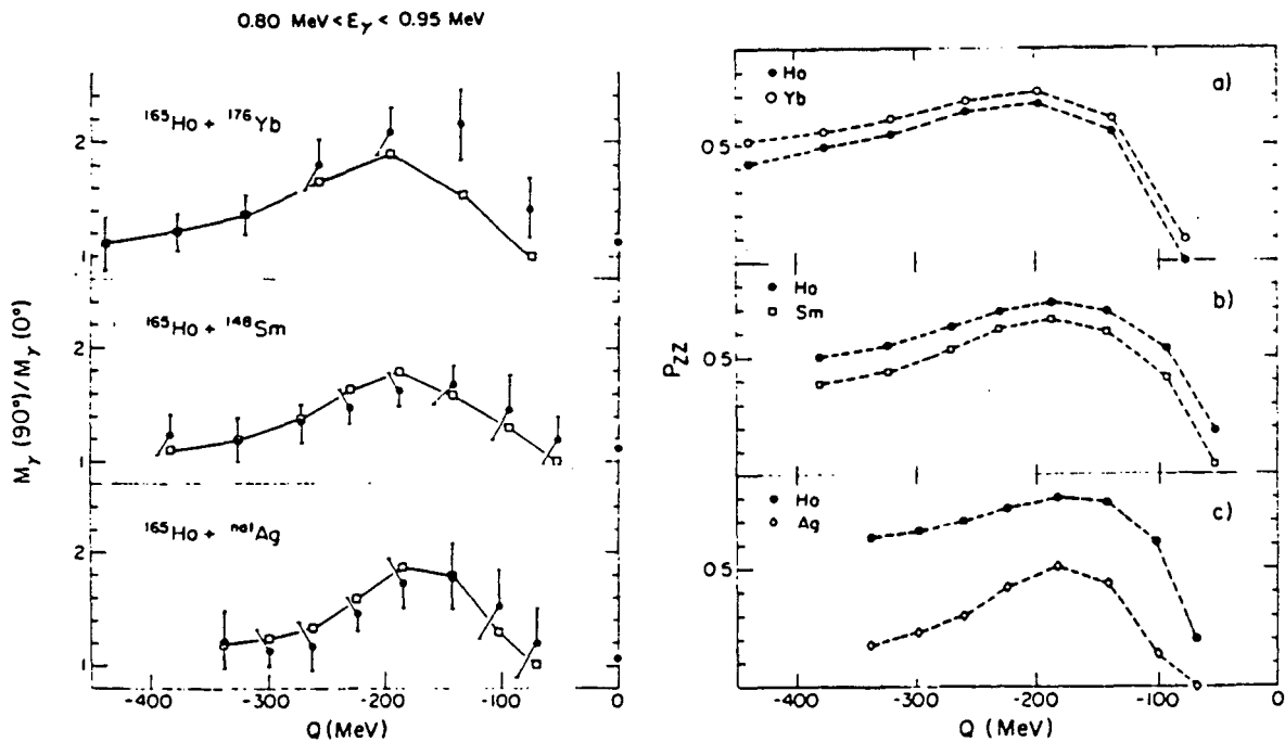
Figure 12. (Left) Comparison between experimental (circles) anisotropies of \gamma -rays ( E = 0.8 - 0.95 \text{ MeV} ) in the reactions 1400 \text{ MeV } ^{165}\text{Ho} + ^{\text{nat}}\text{Ag} , ^{148}\text{Sm} and ^{176}\text{Yb} 20 and a calculation based on the equilibrium statistical model (squares) as a function of Q value. Lines are drawn through the calculated points to guide the eye. (Right) Alignment parameter P_{zz} as a function of Q value, for each of the two inelastic fragments.
