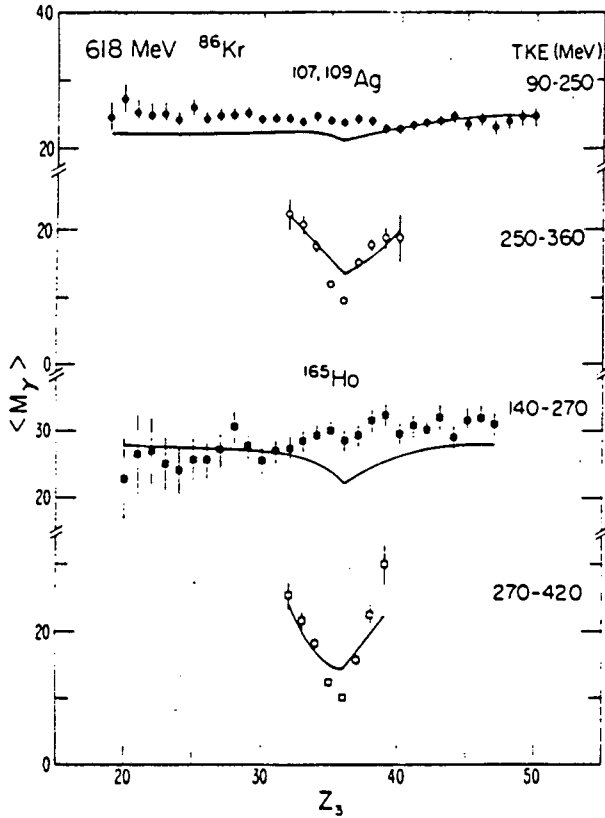
Figure 8. M_Y vs. atomic number for the reactions 618 MeV ^{86}\text{Kr} + \text{natAg} and 618 MeV ^{86}\text{Kr} + ^{165}\text{Ho} . The full and the open symbols are data for a TKE gate on the deep inelastic and quasi-elastic reactions, respectively. The curves are diffusion model calculations 61 .
