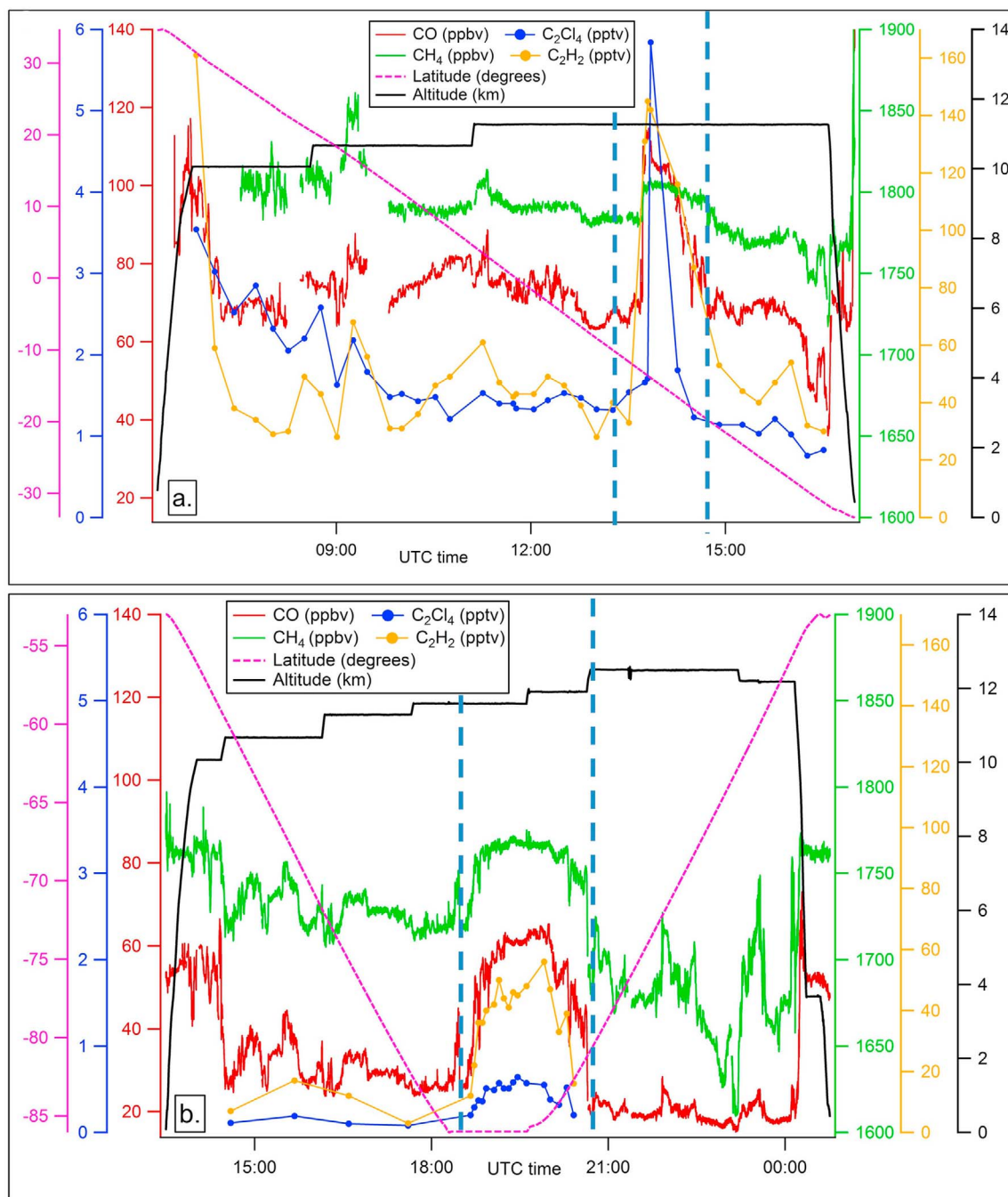
Figure 2. Time series of CO, CH 4 , C 2 Cl 4 , and C 2 H 2 during the (a) transit flight on 12 October 2009 over the South Pacific Ocean and (b) the local flight out of Punta Arenas, Chile, to 86°S on 25 October 2009.
