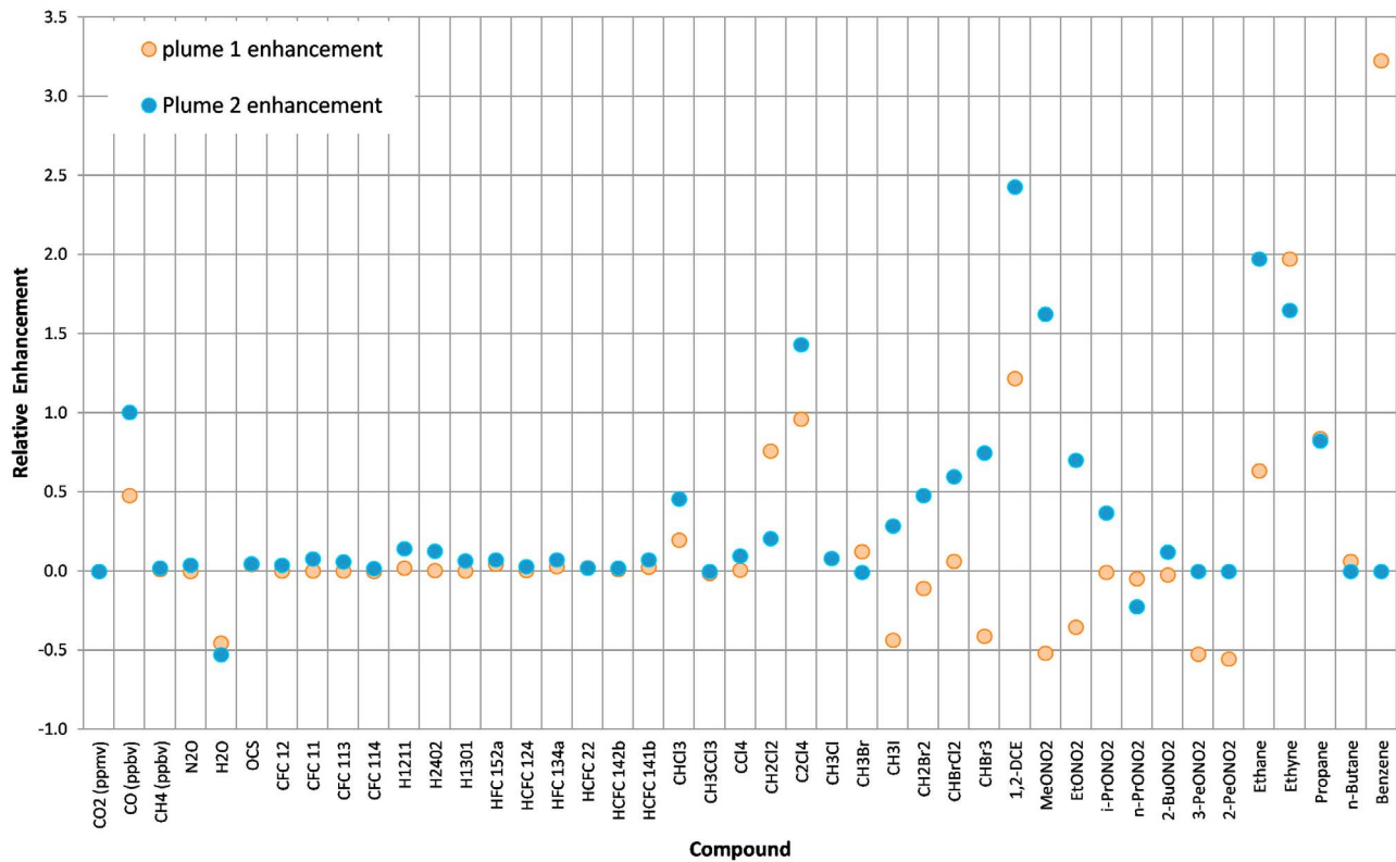
Figure 3. Relative mean enhancements and depletions for the speciated compounds measured in plume 1 (during the transit) and plume 2 (during local 6).
