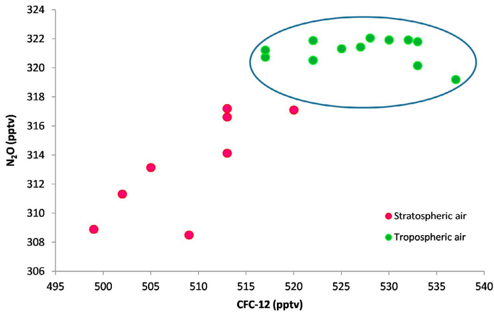
Figure 5. N 2 O and CFC-12 from WAS during the 25 October flight.
