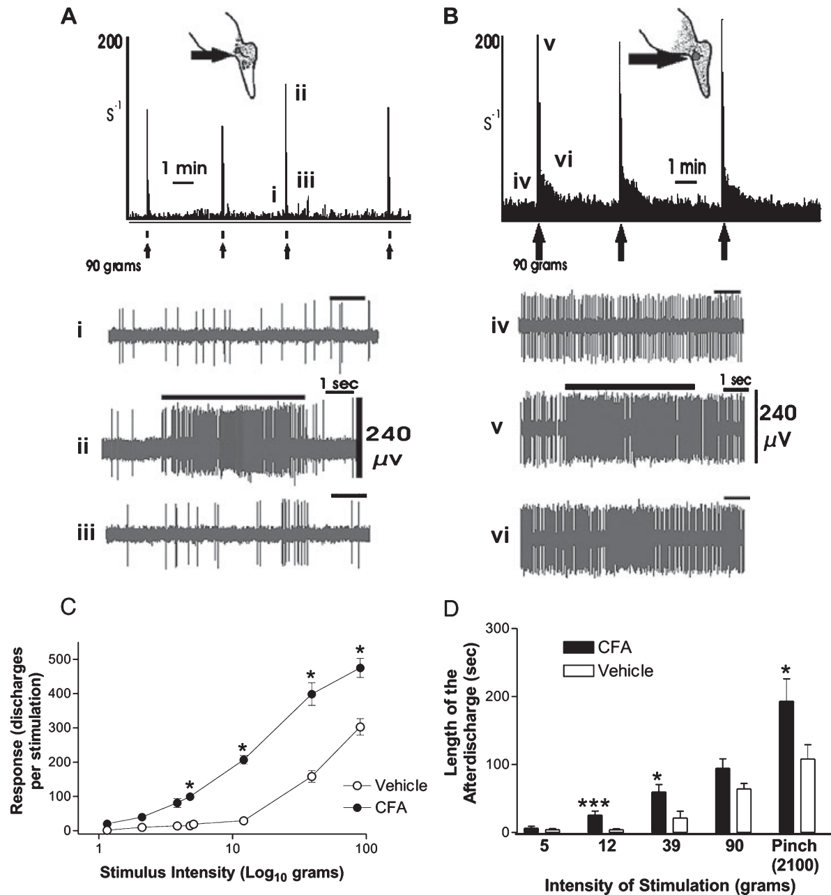
FIG. 3. Electrophysiological data of arthritic animals. Ratemeter histograms in (A) and (B) illustrate recordings from single WDR neurons in control and monoarthritic rats, respectively. Upward arrows indicate times of 5-s applications of 90-g stimuli to the respective cutaneous receptive fields. Larger horizontal arrows in the insets indicate the respective sites of application of the stimuli and the hatched areas indicate the cutaneous receptive fields. (i–vi) Oscilloscope records illustrate the extracellular spike discharges recorded from the neurons illustrated in A and B, taken at the times indicated in the ratemeter histograms; the long horizontal bars above (ii) and (v) indicate the periods of the 5-s stimulation. Data in (C) and (D) illustrate cumulative data from parametric studies in control ( n = 9 ) and monoarthritic rats ( n = 6 ) following either von Frey hair application or pinch (2100 g). Data are expressed as mean \pm SEM with *P < 0.05 and ***P < 0.001 .
