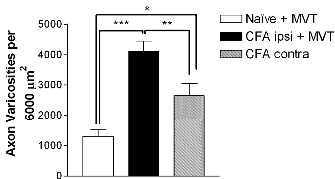
FIG. 6. Quantification of SP immunofluorescent labeling in the superficial dorsal horn of naive and CFA-injected rats. Note the increase in SP labeling in the ipsilateral spinal cord of CFA-injected rats compared to the contralateral side of CFA-injected rats and to control animals: * P < 0.05 , ** P < 0.01 , *** P < 0.001 .
