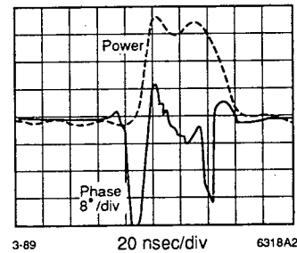
FIG. 3. Measurement of RF power and phase in the SHARK/TW relativistic klystron. Stability of the phase-amplitude product (solid trace) is maintained to within 16^\circ during the 35 nsec period of 60-MW peak RF amplitude (dashed trace).
