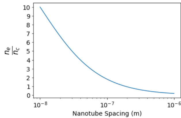
Figure 7. Ratio of perceived electron density to critical density n_e/n_c as a function of the vacuum spacing between CNTs. (Note that this ratio is the reciprocal of that quoted in previous sections.) The density inside a CNT is 10^{22} \text{ cm}^{-3} , and the width of a CNT is 10 nm. The laser wavelength is 1 micron.
