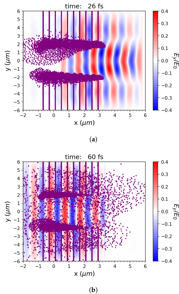
Figure 8. Example of simulation results with first laser extracting electrons from the CNTs (a) and a second pulse accelerating the extracted electrons (b). The purple dots indicate the locations of individual electrons, and the colormap indicates the strength of the laser field. The laser field is normalized to the nominal peak amplitude E_0 \approx 1.6 \times 10^{12} \text{ V/m} .
