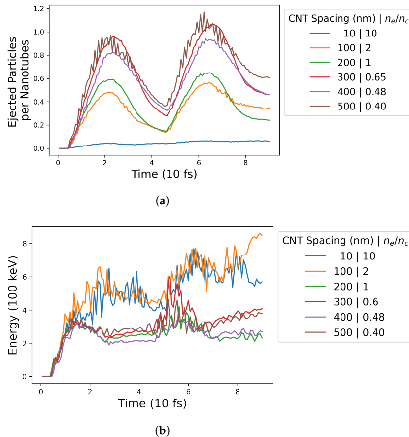
Figure 10. Number of extracted electrons (a) normalized to total number of CNTs in the simulation as a function of time and maximum energy of electrons (b) over simulation time for various values of CNT spacing. The first laser reaches CNTs in the first few femtoseconds. The second laser reaches the CNTs at around 45 fs. The laser intensity is a_0 = 0.5 .
