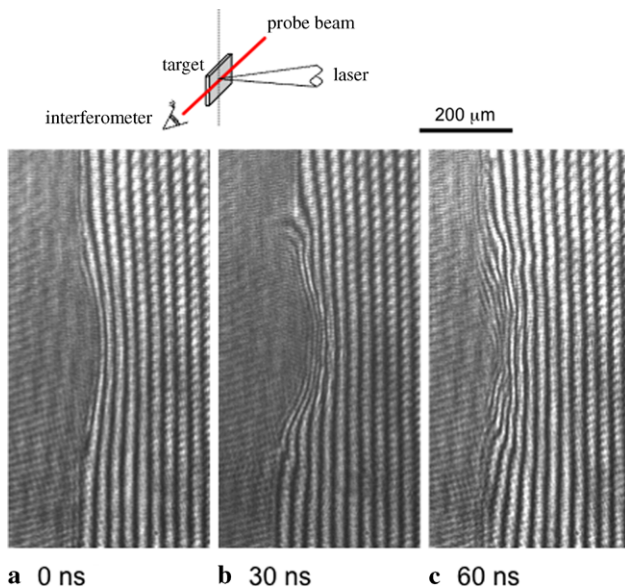
Fig. 1 Interferograms of Sn plasma irradiated with \text{CO}_2 laser pulse observed at various delay times of (a) 0, (b) 30, and (c) 60 ns with respect to the peak of the laser pulse
