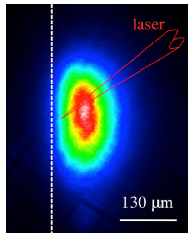
Fig. 4 In-band EUV image of Sn plasma irradiated with CO 2 laser pulse incident at an angle of 45 degrees respect to the target normal
