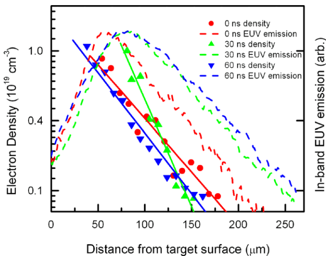
Fig. 3 Profiles of plasma density and in-band EUV emission along the line of laser incidence at various delay times 0, 30, and 60 ns
