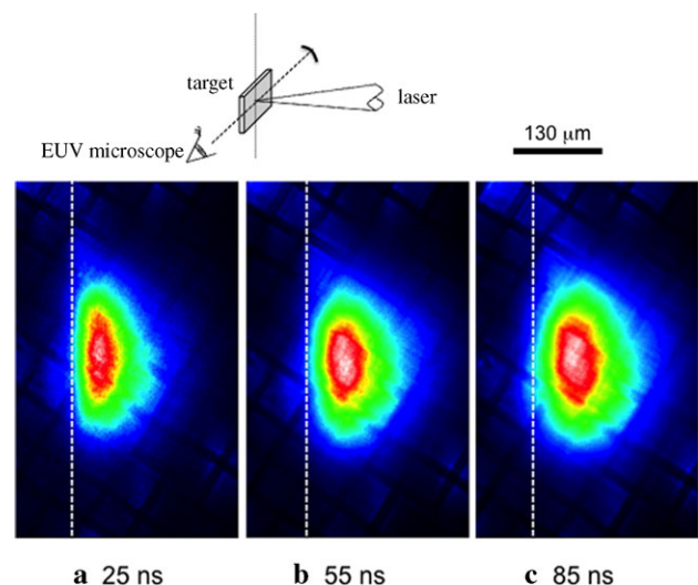
Fig. 2 In-band EUV images of Sn plasma irradiated with \text{CO}_2 laser with various pulse durations of (a) 25, (b) 55, and (c) 85 ns
