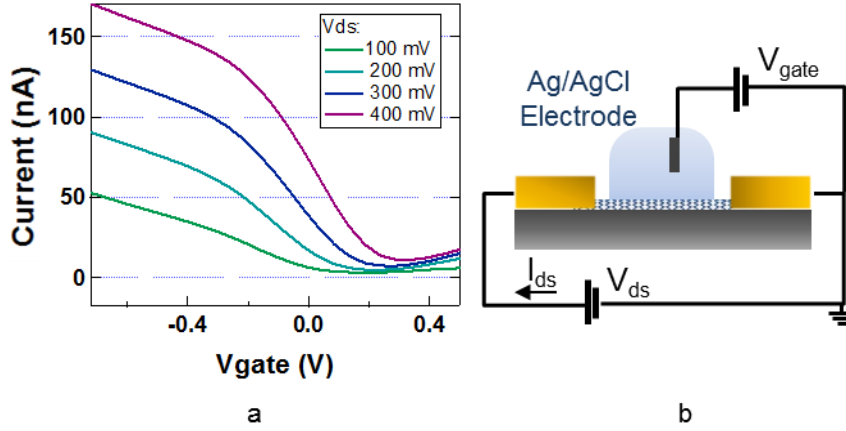
Figure 4.2. DC characterization of the device. (a) Drain-Source current vs. (electrolyte) gate voltage for a 3\ \mu\text{m} \times 3\ \mu\text{m} device at different applied drain-source voltages. (b) Schematic showing the DC measurement set-up.
