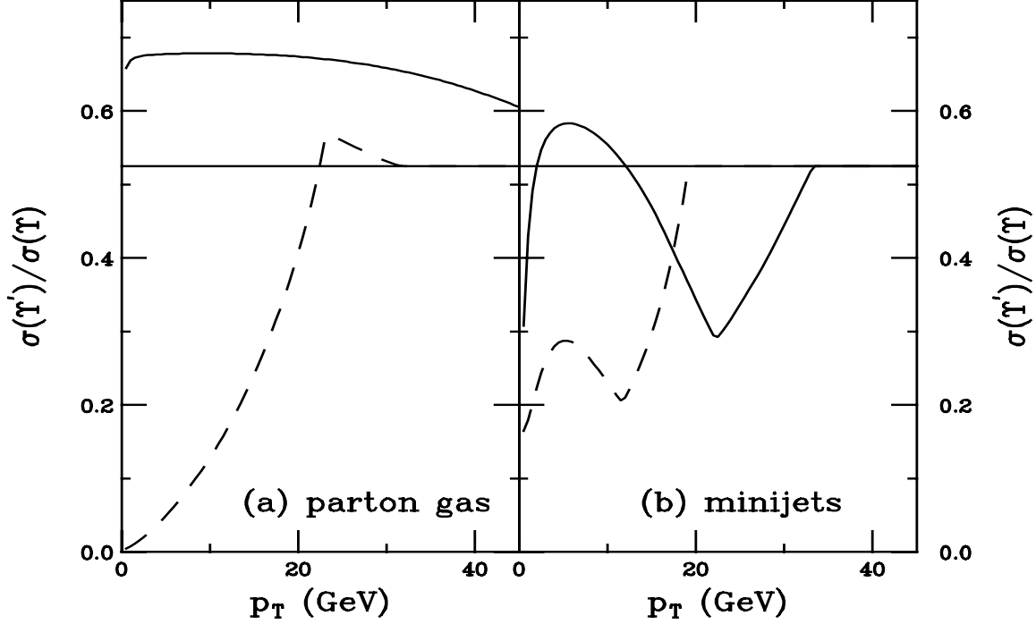
Figure 2. The \Upsilon'/\Upsilon ratio computed from Eq. (1) is shown for the initial conditions in Table 3 with R = R_{\text{Pb}} . In (a), parton gas results are shown for \mu \propto gT (dashed) and \mu = 4T (solid). In (b) minijet results are given for \mu = 4T without shadowing (solid) and with HPC shadowing (dashed). The horizontal curve represents the pp ratio. From [16].
