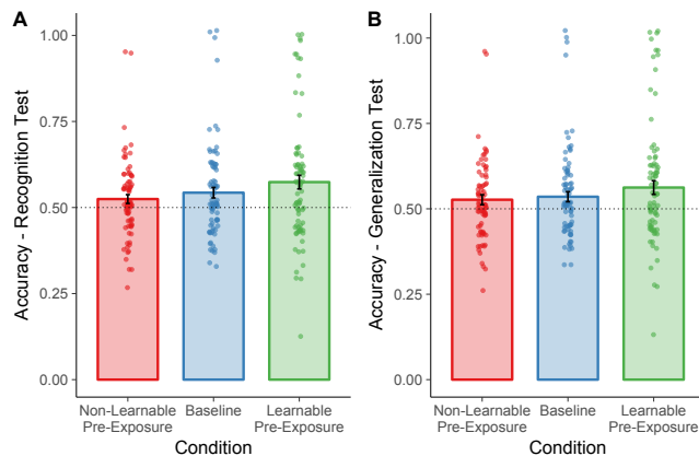
Figure 6: (A) Recognition and (B) Generalization Test Accuracy in Experiment 2. Error bars represent \pm 1 SEs.
