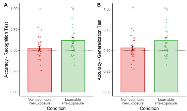
Figure 4: (A) Recognition and (B) Generalization Test Accuracy in Experiment 1. Error bars represent \pm 1 SEs.
