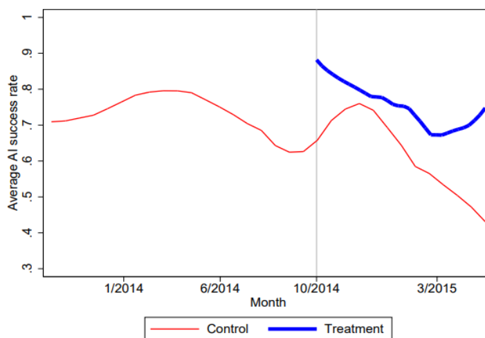
Figure 4: AI success rates in real time—clearinghouse data
