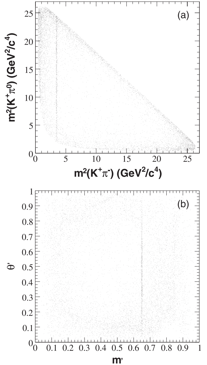
FIG. 1. The standard (a) and square (b) Dalitz plots of the selected data sample of 8014 events. The structures are more spread out in the square Dalitz plot. The \bar{D}^0 \rightarrow K^+ \pi^- narrow band is preserved with the choice made for the m' variable.
