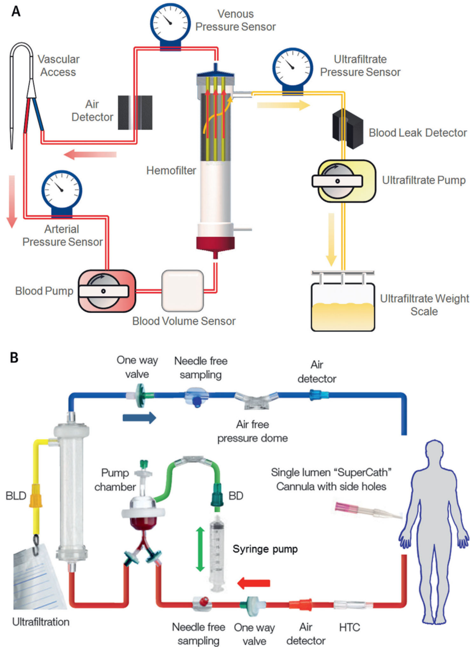
FIGURE 1. UF Circuit
