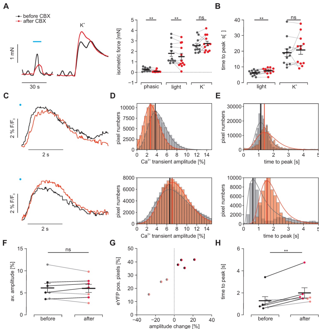
Figure 5. Effects of electrical coupling via gap junctions. To block electrical coupling via connexins, we applied 30 \mu M carbenoxolone (CBX, red) for at least 15 min in gastric antrum strips from ChR2 animals. (A) Representative traces (left) and aggregated data (right, N = 4, n = 12) of isometric force measurements. Contractions were spontaneous-phasic, induced by blue light (blue bar, 10 s, 0.2 mW/mm 2 ) or 60 mM K + . Statistical analysis was performed with 2-way repeated measures ANOVA with Sidak's multiple comparison test (p = 0.003 for Phasic, p = 0.008 for Light, p = 0.54 for K + ). (B) Analysis of time to peak (N = 4, n = 12). Statistical analysis was performed with 2-way repeated measures ANOVA with Sidak's multiple comparison test (p = 0.003 for Light; p = 0.63 for K + ). C-H. Macroscopic Ca 2+ imaging of antral smooth muscle strips following stimulation with blue light (11 mm 2 , 50 ms, 6 mW/mm 2 ). (C) Original traces of tracked ROIs before (black) and after (red) CBX. Illumination indicated by blue dot. In the upper example, note the decreased amplitude and the prolonged time to peak, in contrast to the lower example with increased amplitude but also prolonged time to peak. (D) Histograms of peak heights (indicated by vertical line) of log-normal fits for light-induced Ca 2+ transient amplitudes (fractional intensity change) of two different strips before and after CBX. Note the overall decrease in amplitude in the upper, and the increase in the lower example. (E) Histograms of peak times (indicated by vertical line) of log-normal fits for the analysis of the time interval between the light pulse and peak. Note the time prolongation in both examples. (F) Comparison of the light-induced average Ca 2+ transient amplitude before and after CBX. Strips with an increasing amplitude are color coded in black/dark red and strips with a decrease in gray/light red. (G) Relationship between the fraction of eYFP positive pixels within the analyzed smooth muscle strip and the change in average amplitude. (H) Comparison of the average time to peak before and after CBX (p = 0.004). In F-H each dot represents a separately analyzed smooth muscle strip (n = 7). Statistical analysis was performed with paired student's t-tests.
