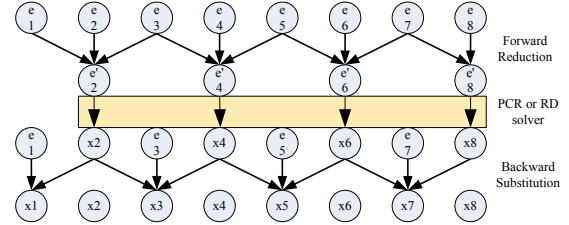
Figure 4. Hybrid algorithms for an 8-unknown system. Letter e stands for equation, and e' stands for updated equation.
