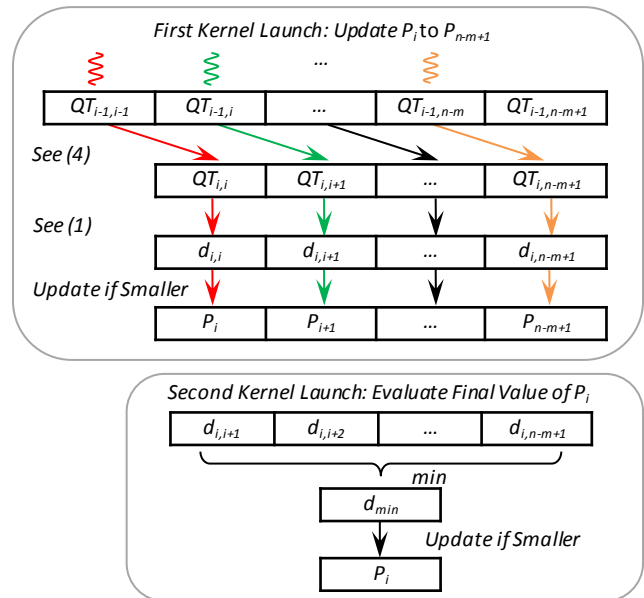
Fig. 6. Modifying the third step of GPU-STOMP. top ) Launch only n-m-i+2 threads (instead of the n-m+1 threads in Fig. 5) this time at the i^{th} iteration. bottom ) Launch another kernel to evaluate the final value of P_i .
