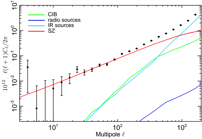
Fig. 15: NIILC - MILCA F/L cross-power spectrum (black) compared to the power spectra of the physically motivated foreground models. The considered foregrounds are: clustered CIB (green line); infrared sources (cyan line); and radio sources (blue line). Additionally, the best-fit tSZ power spectrum model presented in Sect. 7.1 is also plotted as a solid red line.
