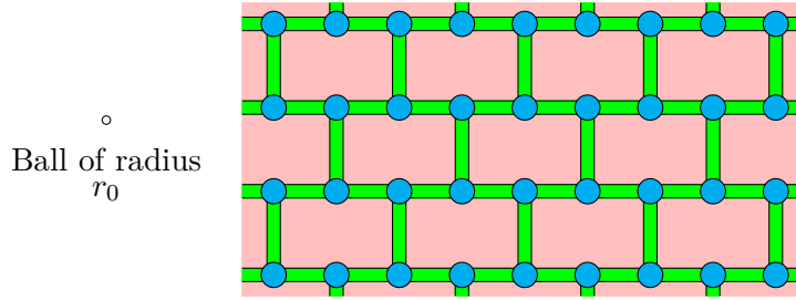
Figure 2: Sets U_0 (pink), U_1 (green), U_2 (blue) satisfying condition (2) when r = r_0 , X = \mathbb{R}^2 , and d = 2 .
