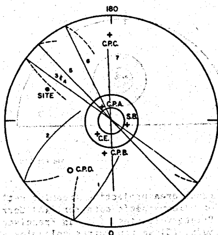
Figure 4. Polar paths for major excursions in Brunhes period: (1) Gothenburg, (2) Starno, (3) Lake Mungo, (4) Laschamp, (5) Lake Biwa, (6) and (7) Blake. Virtual geomagnetic poles for Cerro Prieto (CPA, CPB, CPC, CPD), Salton Buttes (SB), and Crater Elegante (CE). (CPD represents pole dike of site 2 at Cerro Prieto with a pole in the southern hemisphere; + southseeking field, 0 northseeking field.
