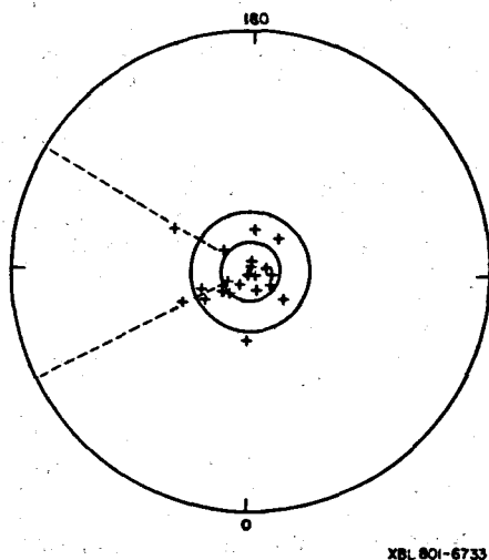
Figure 5. Quaternary virtual geomagnetic poles for western United States (Irving et al., 1976).
