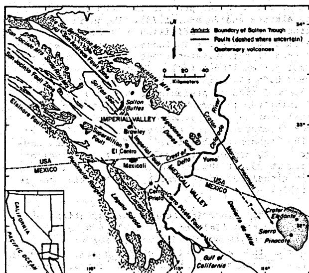
Figure 1. Location of sampling areas in the Salton Trough.
