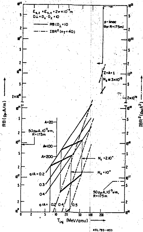
Fig. 4 Linac brightness B (solid lines), current-brightness product IB (dashed lines), multiplied by R, R 2 respectively, as required to reach space charge limit N s in synchrotron for A = 200. Assumed is total transverse dilution D T = D x · D y · D z = 10, number of injected turns = 40, horizontal and vertical acceptance = 2π · 10 -5 m. Heavy solid lines correspond to N s = 2 · 10 11 and 10 11 respectively.
