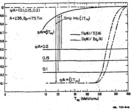
Fig. 5 Solid lines indicate kinetic energy obtainable with given q/A, with and without stripping at linac exit normalized to T(Z/A). Dashed lines indicate corresponding intensity, normalized to intensity obtained without stripping.
