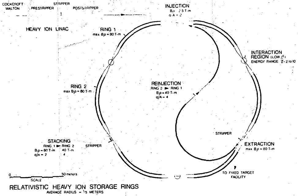
Fig. 3 Accelerator/Storage ring concept from preliminary LBL-studies. B\rho assumed in this paper is 175 \mu\text{m} , B_{\text{max}} = 5\text{T} , \bar{B} = 1\text{T}
