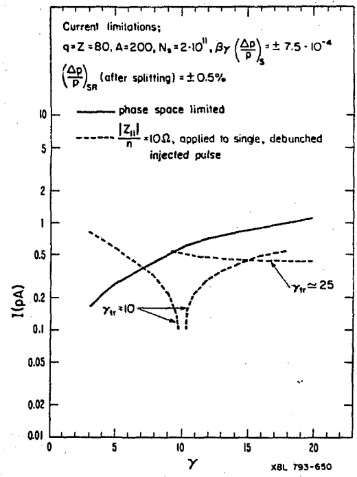
Fig. 7 Current limitations from longitudinal stability considerations (dashed lines), from linac momentum spread (solid lines).
