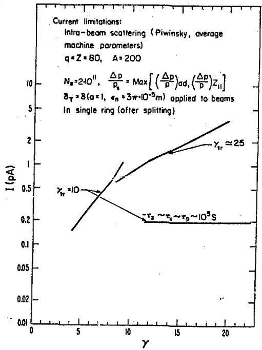
Fig. 8 Current limitations from intra-beam scattering.
