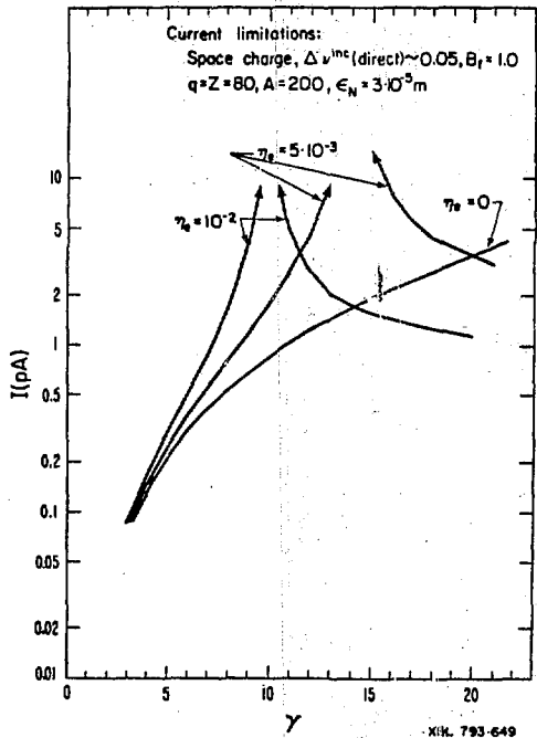
Fig. 6 Space charge limited currents for parameters indicated in figure.
