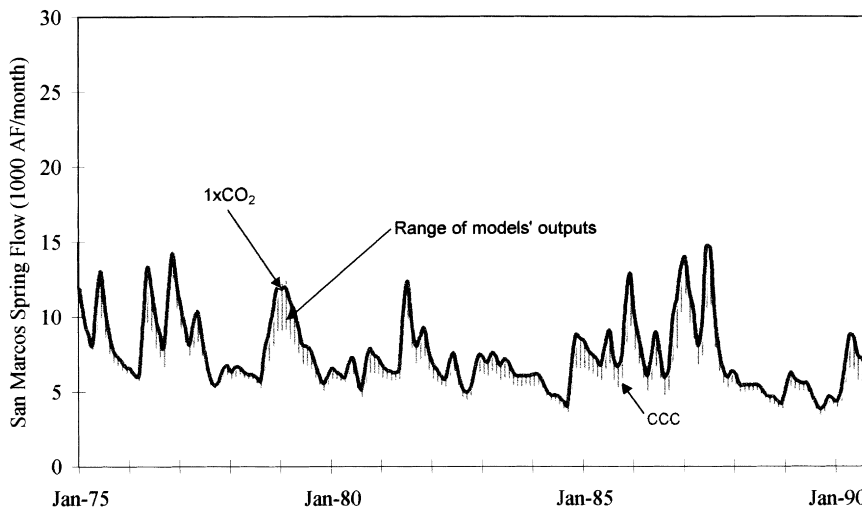
Fig. 10. Range of San Marcos spring flow predictions from six GCMs' scaling factors (1975–1990 base period of above-average recharge; 1 AF = 1233 m 3 ).
