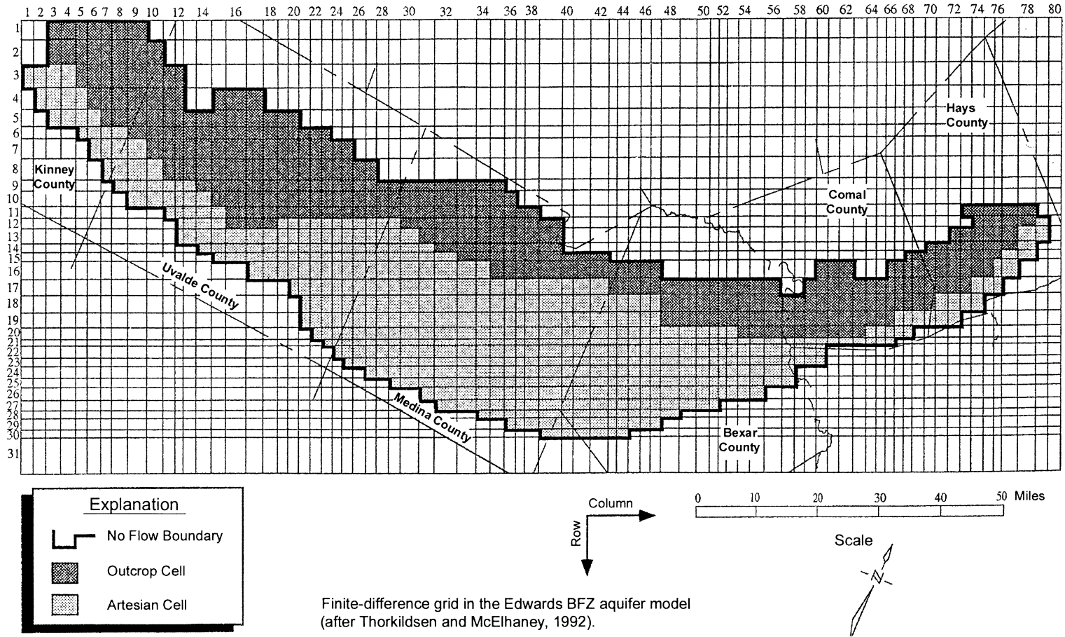
Fig. 2. Finite-difference grid for the Edwards BFZ aquifer (after Thorkildsen and McElhane, 1992; see Fig. 1 for location of grid relative to surrounding counties in the study area).
