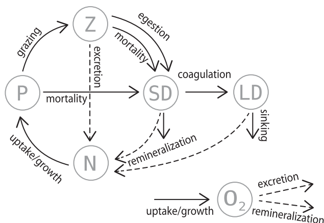
Figure 2. Schematic of the Cascadia ecosystem model. Circles represent pools of nitrogen in the form of dissolved inorganic nitrogen (N), phytoplankton (P), zooplankton (Z), small detritus (SD), large detritus (LD), and oxygen (O 2 ). Arrows represent fluxes of nitrogen between the pools.
