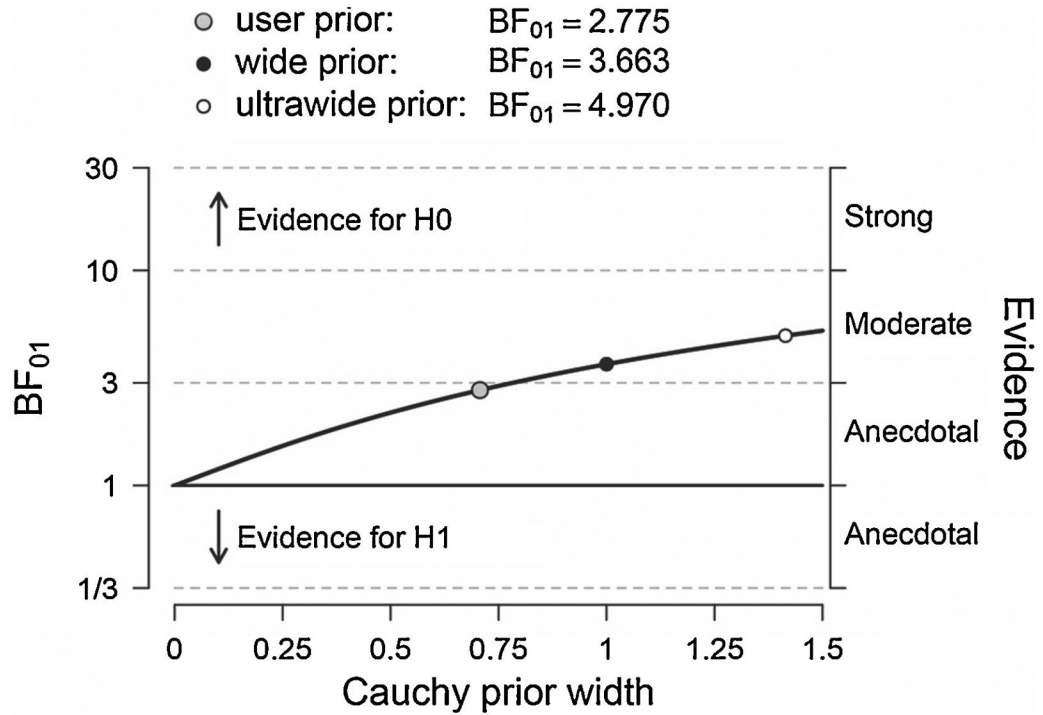
Figure 2. Graph showing how the width ( r value, shown on the X axis) of different prior distributions influences Bayes Factor scores (BF, shown on Y axis) from the Bayesian t-test results. Here the “user prior” is JASP’s default Cauchy distribution ( r=.707 ) yields relative evidence in favor of the null hypothesis that is below BF=3 , while the more standard Jeffreys’ prior ( r=1 ) is greater than three, indicating evidence analogous to a moderate effect. Data shown is from the interpersonal distance task in which we tested the effects of receiving AVP versus PLA nasal sprays on the change in female participants’ trustworthiness judgments between faces that appeared nearby and far away.
