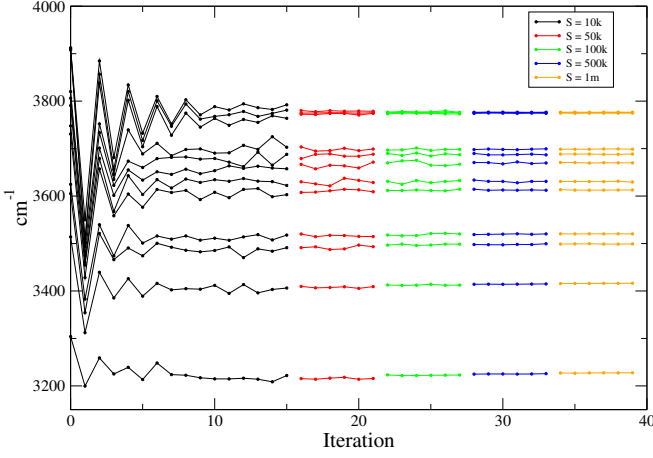
FIG. 2. The OH stretch fundamental frequencies of MB-pol hexamer prism at T = 0 , computed by the SCP method using a single grid for integration. The frequencies are shown as a function of the iteration number. Different colors correspond to different numbers of points, S , in the Sobol sequence used to compute the Gaussian integrals.
