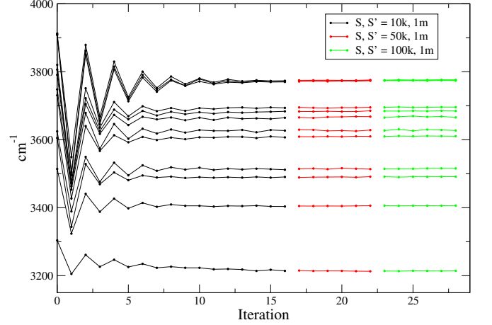
FIG. 4. Two grid SCP calculation at T = 0 for the MB-pol hexamer prism. S and S' indicate the numbers of gradient evaluations for, respectively, MB-pol and q-TIP4P/F PEF's.
