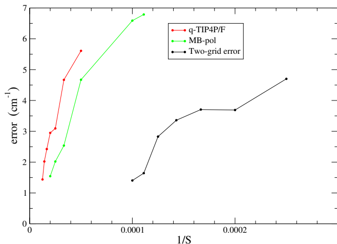
FIG. 6. The error for the computed fundamental frequencies of hexamer prism averaged over the 12 OH stretch modes as a function of 1/S . The errors were computed by taking the difference with the frequencies computed using S = 2.5 \times 10^6 . Red line: using a single grid SCP calculation for the q-TIP4P/F hexamer.
