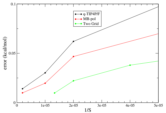
FIG. 8. Same as Fig. 6 but for the Helmholtz free energy, which at T = 0 is equal to the ground state energy of the optimal harmonic system as obtained by SCP.
