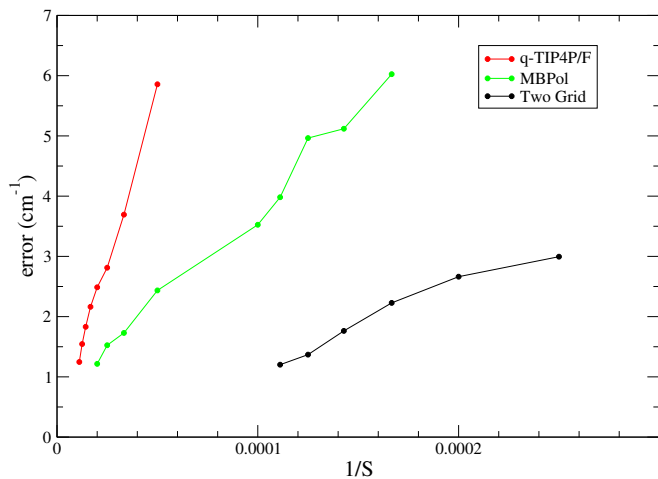
FIG. 7. Same as Fig. 6 but averaged over all the (3N - 6) fundamental frequencies of water hexamer.
