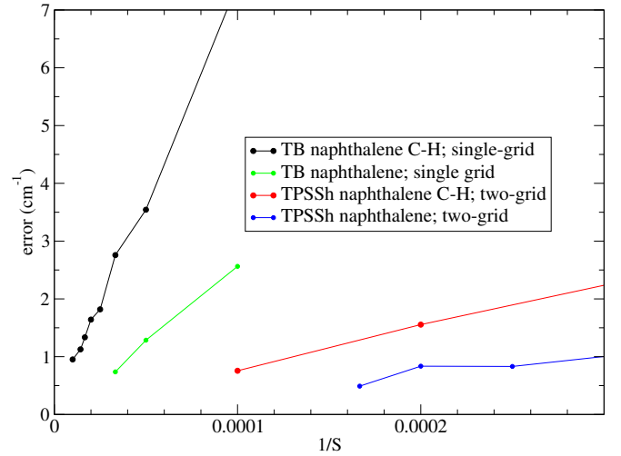
FIG. 11. The errors for the computed fundamental frequencies of naphthalene averaged over the 8 CH stretch modes as a function of 1/S and over all the (3N - 6) fundamental frequencies of naphthalene. The errors were computed by taking the difference with the frequencies computed using S = 10^6 for the TB naphthalene (single-grid SCP) and S = 4 \times 10^4 ; S' = 10^6 , for the TPSSh naphthalene (two-grid SCP).
