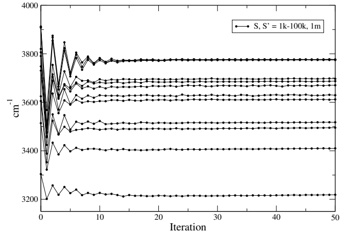
FIG. 5. Two grid SCP calculation for the MB-pol hexamer prism as in Fig. 4 but using the quadratic schedule S = (10^5 - 10^3) \times (0.02i)^2 ( i = 1, \dots, 50 ) with fixed S' = 10^6 .
