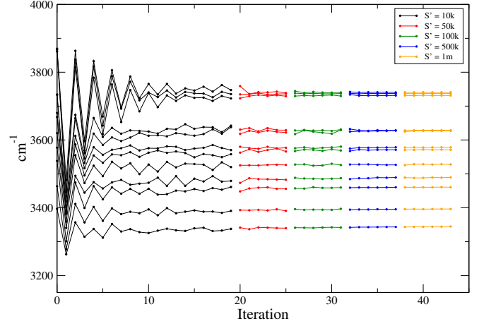
FIG. 3. Same as Fig. 2 but for the q-TIP4P/F hexamer prism.
